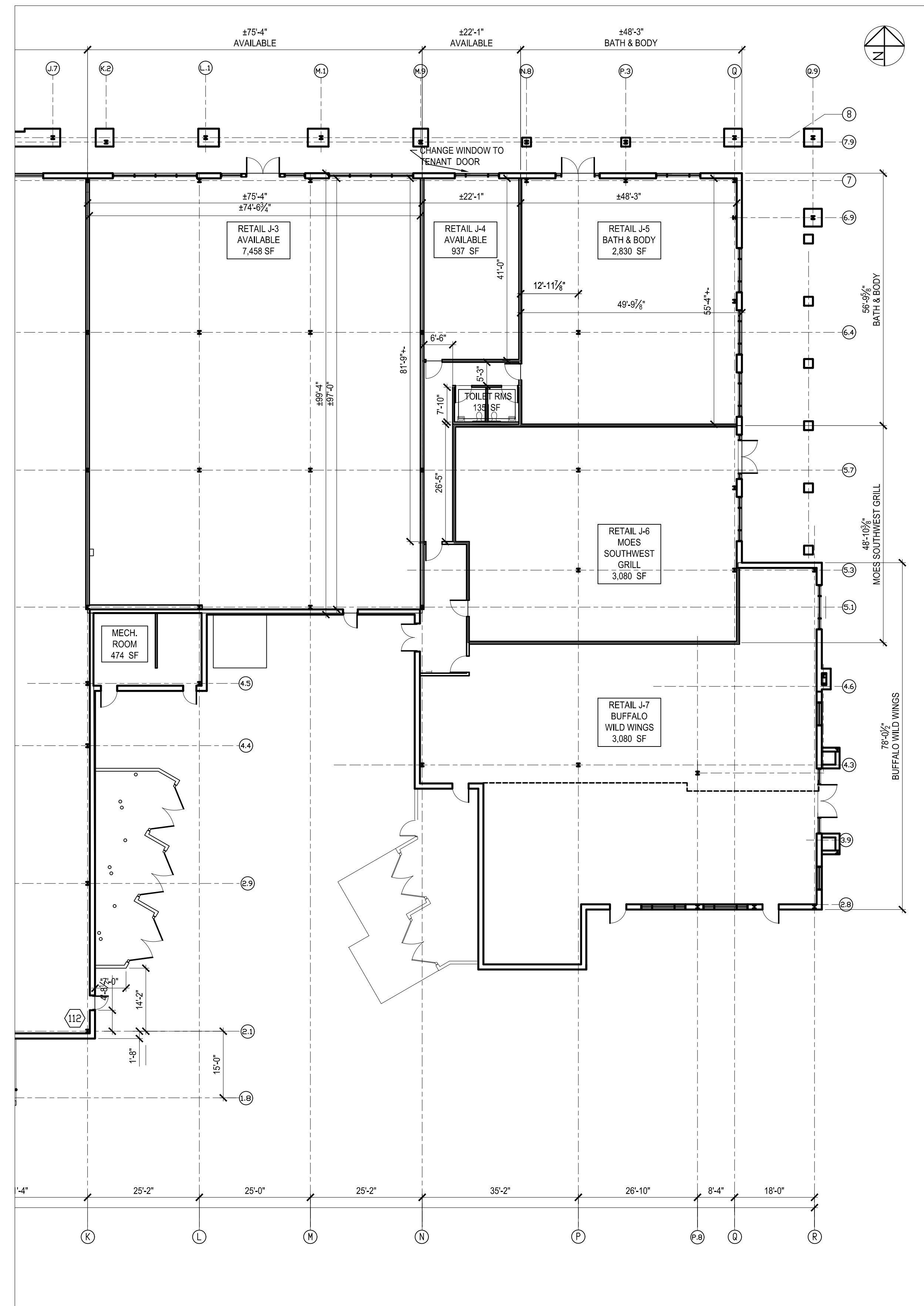
PARTIAL FLOOR PLAN
