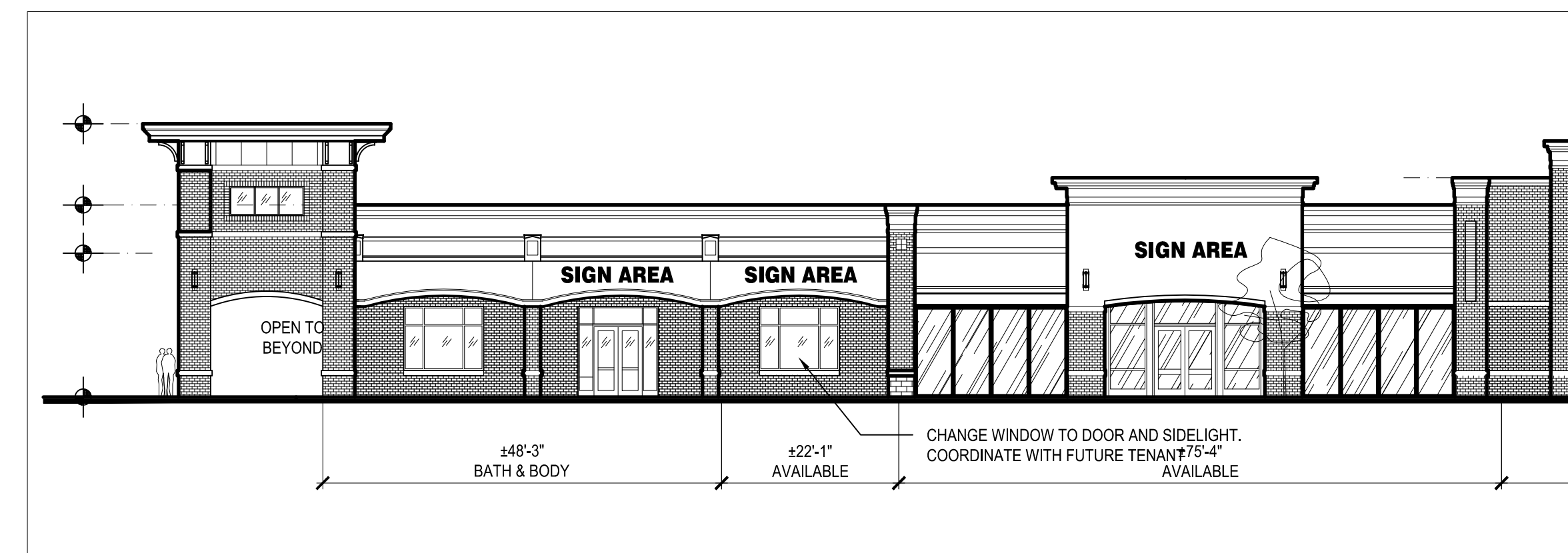
PARTIAL FRONT ELEVATION
