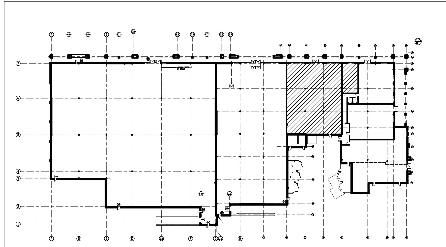
KEY PLAN
