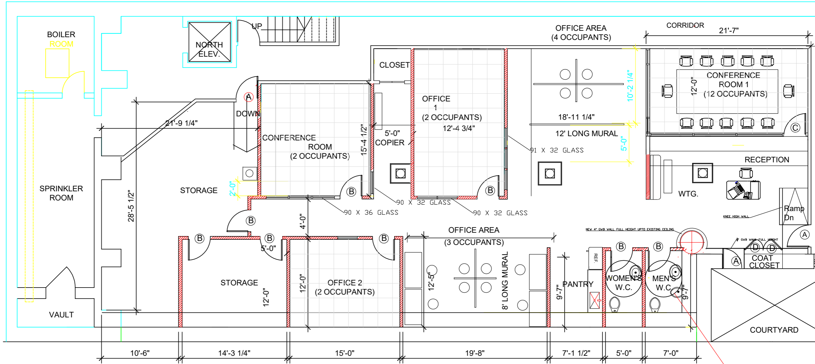
CELLAR PLAN Scale \frac{1}{8}'' = 1'-0''
