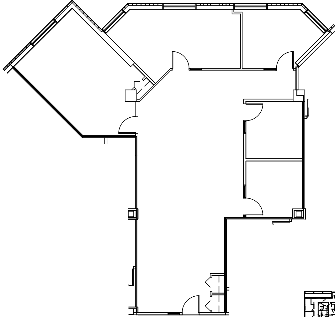
SUITE 235 - FLOOR PLAN 3/32" = 1'-0"
