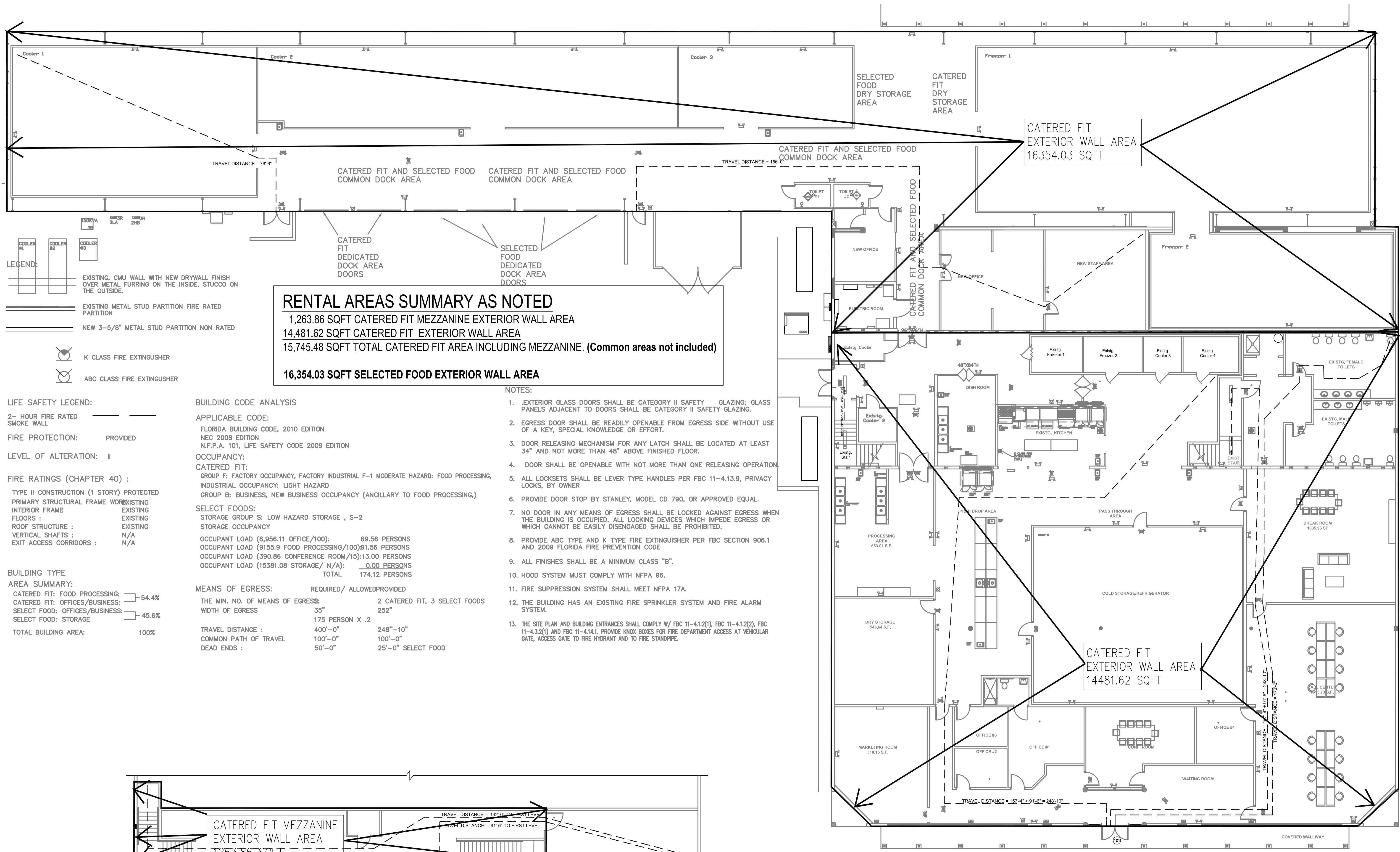
LIFE SAFETY FIRST FLOOR PLAN SCALE: 1" = 10'-0"
