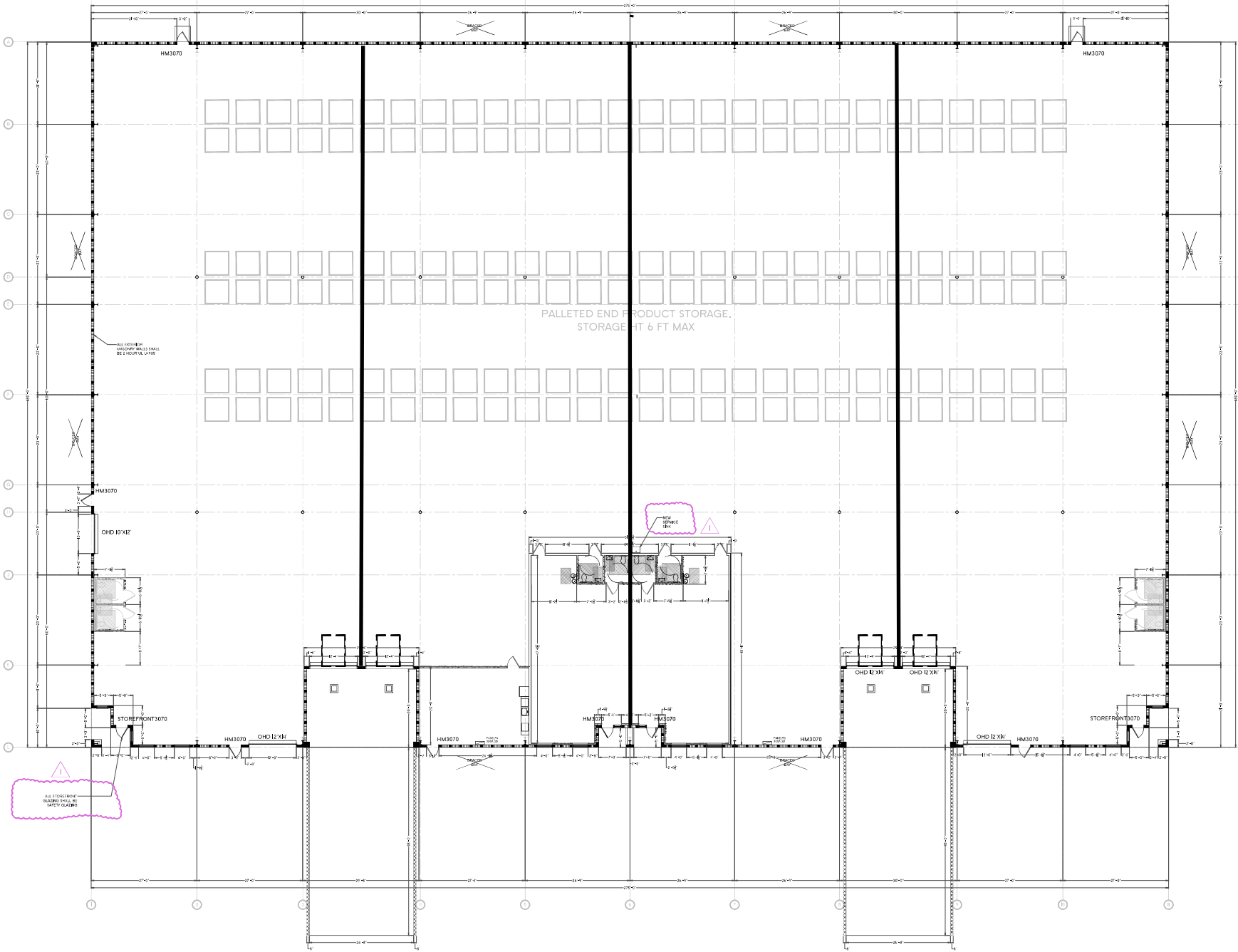
PROPOSED FLOOR PLAN SCALE: 3/32"=1'-0"
