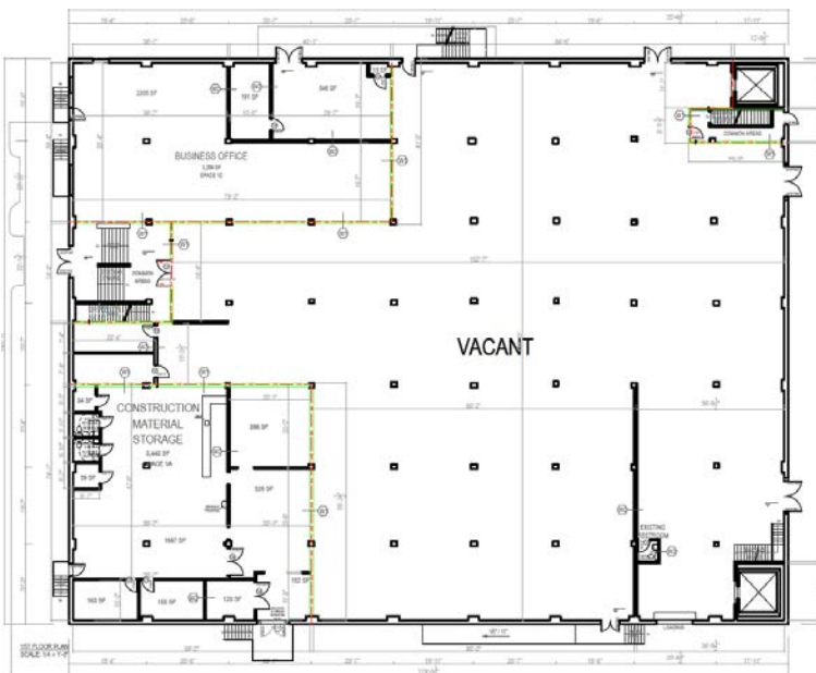
1st Floor
