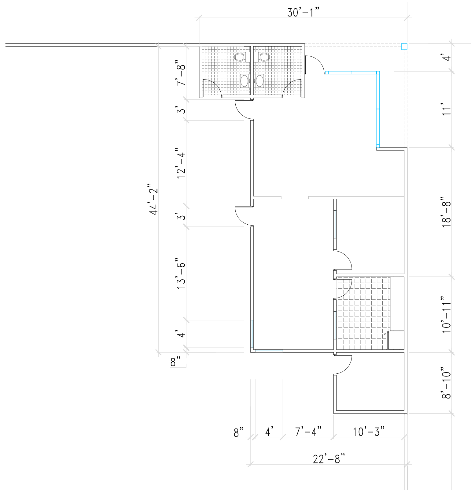
2 BLDG#4971 SUITE A FLOOR PLAN
