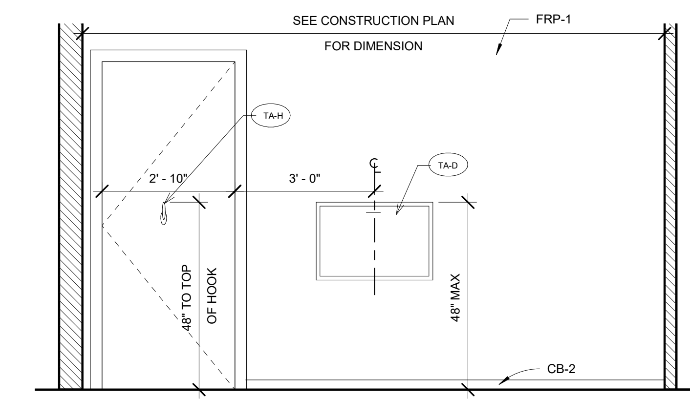
8 WOMENS HANDICAP BATHROOM ELEVATION 8 1/2" = 1'-0"
