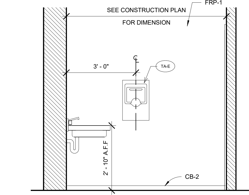
7 WOMENS HANDICAP BATHROOM ELEVATION 7 1/2" = 1'-0"
