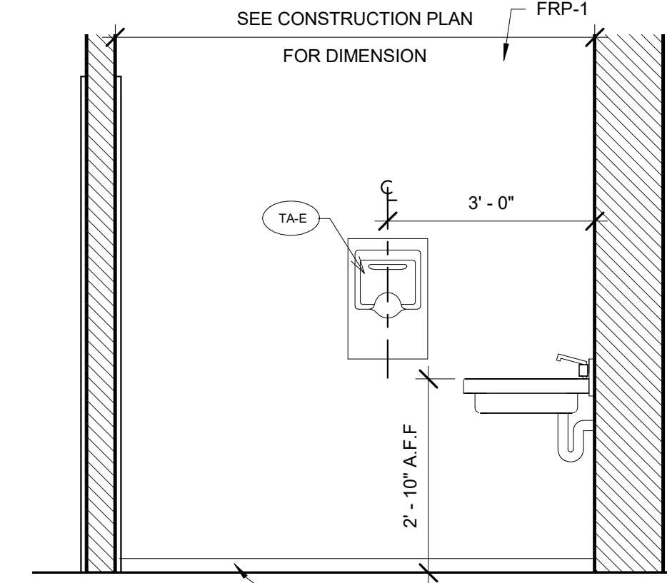
4 MENS HANDICAP BATHROOM ELEVATION 4 1/2" = 1'-0"
