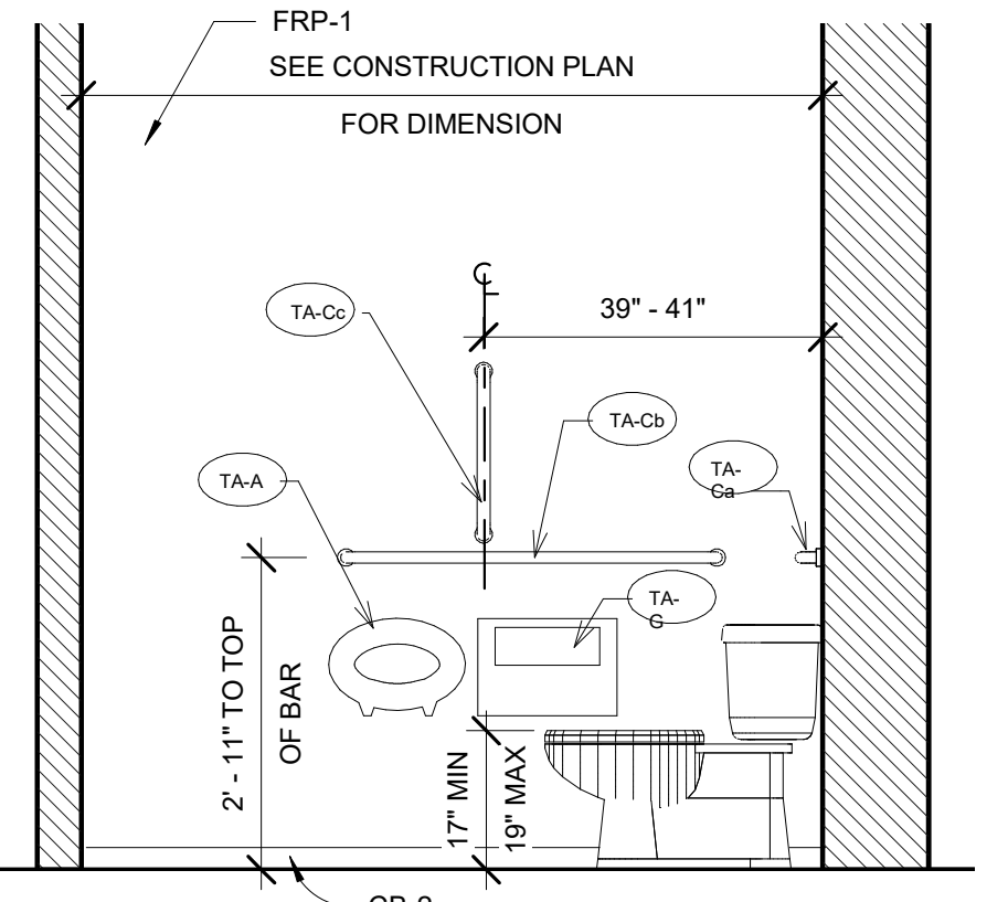
10 WOMENS HANDICAP BATHROOM ELEVATION 10 1/2" = 1'-0"
