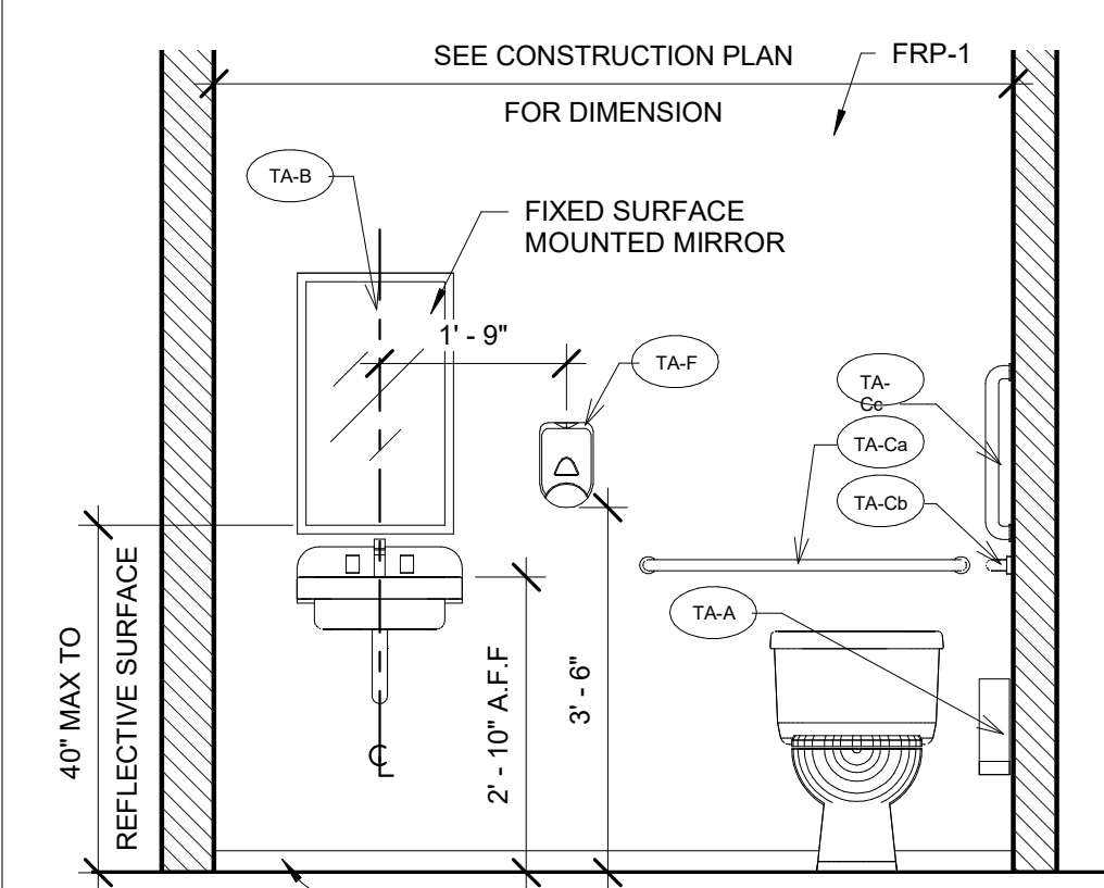
5 MENS HANDICAP BATHROOM ELEVATION 5 1/2" = 1'-0"
