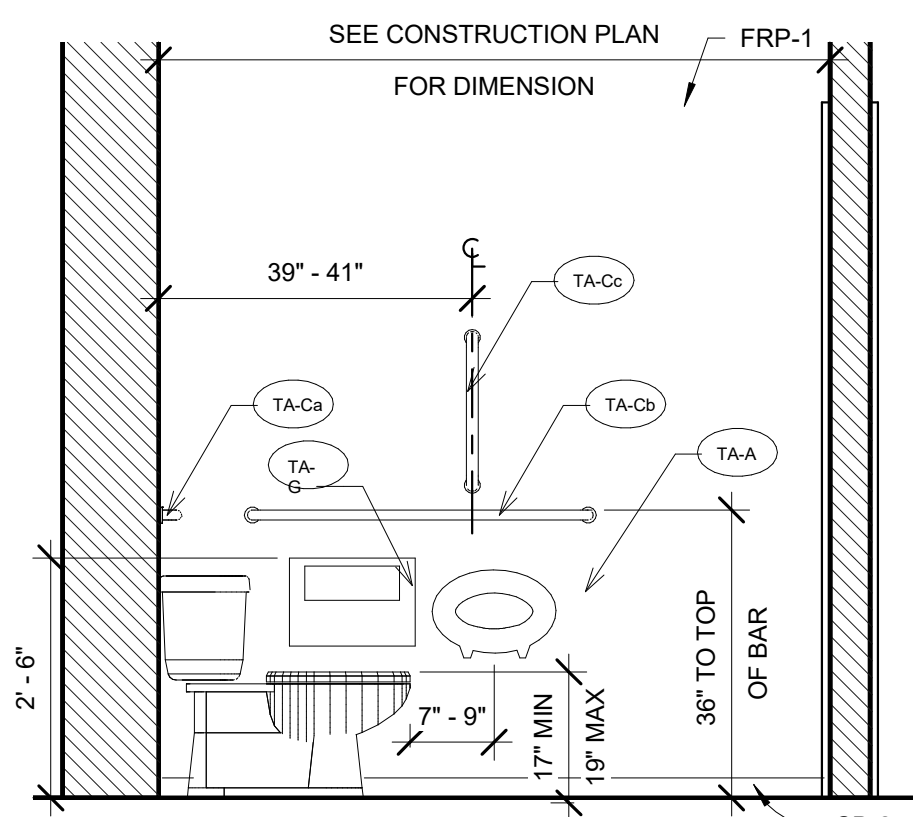
6 MENS HANDICAP BATHROOM ELEVATION 6 1/2" = 1'-0"
