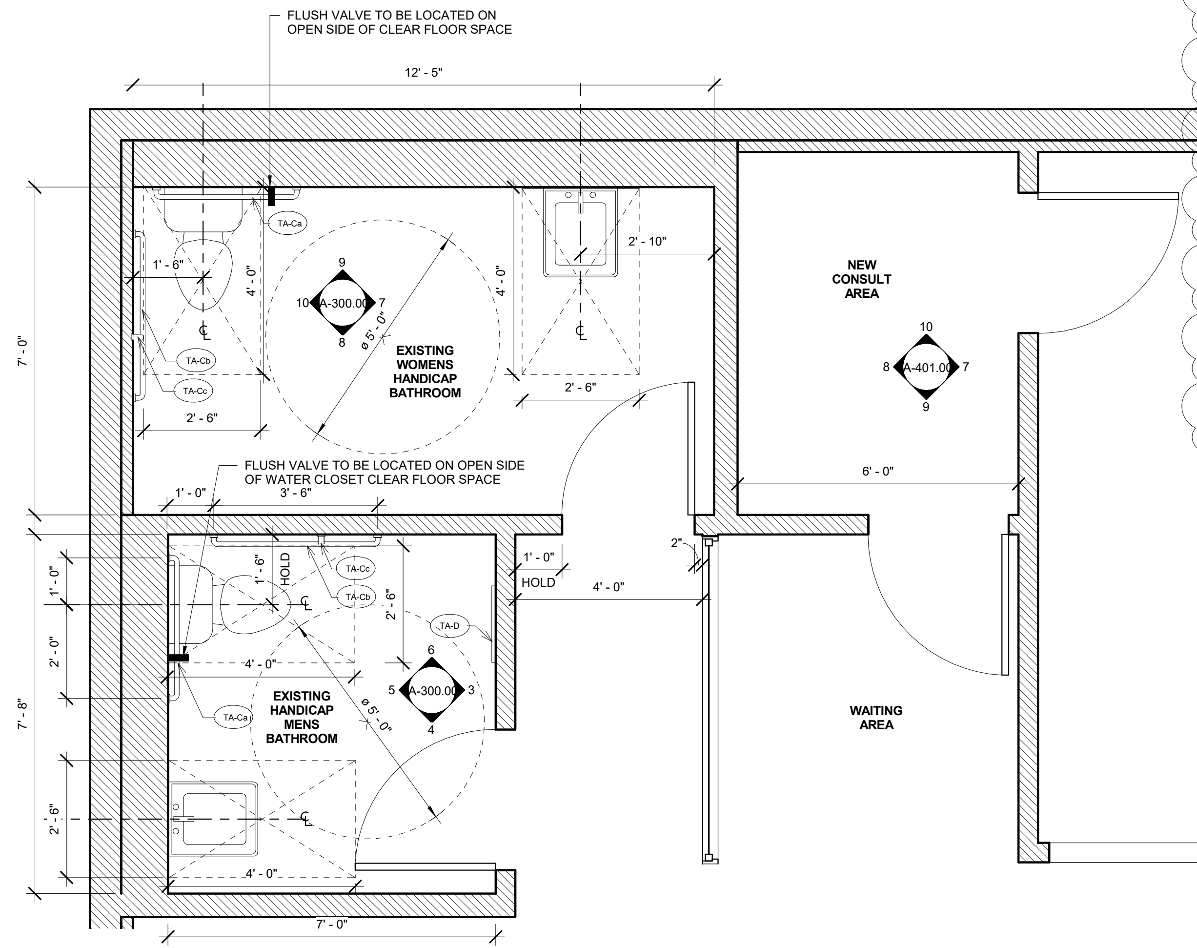
1 ENLARGED HANDICAP MENS/WOMENS BATHROOM PLAN 1/2" = 1'-0"
