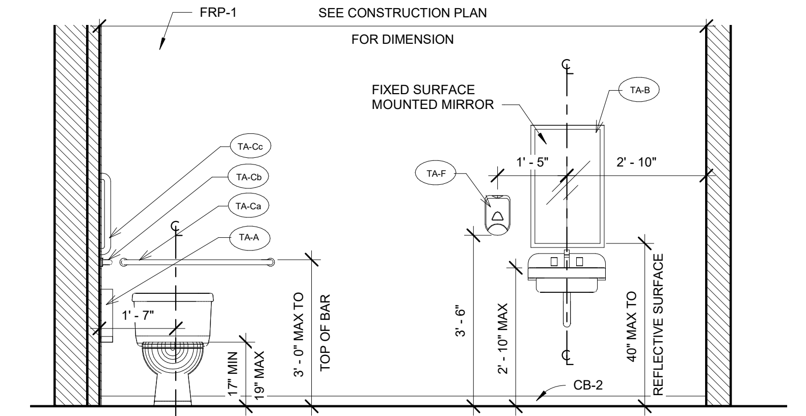
9 WOMENS HANDICAP BATHROOM ELEVATION 9 1/2" = 1'-0"
