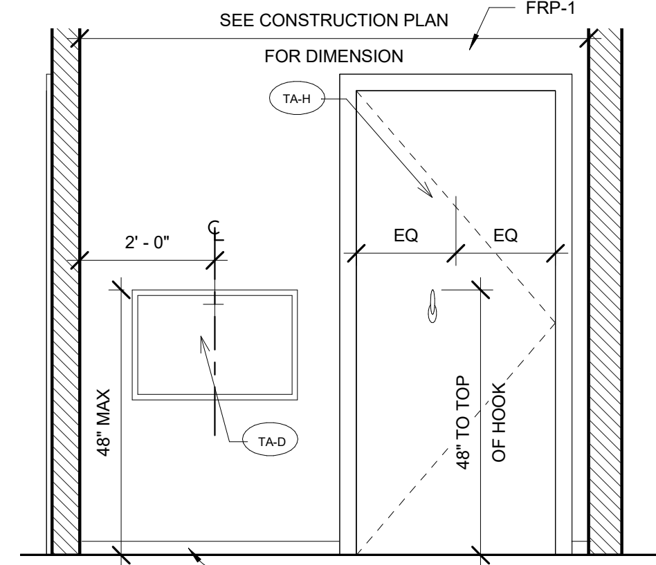
3 MENS HANDICAP BATHROOM ELEVATION 3 1/2" = 1'-0"
