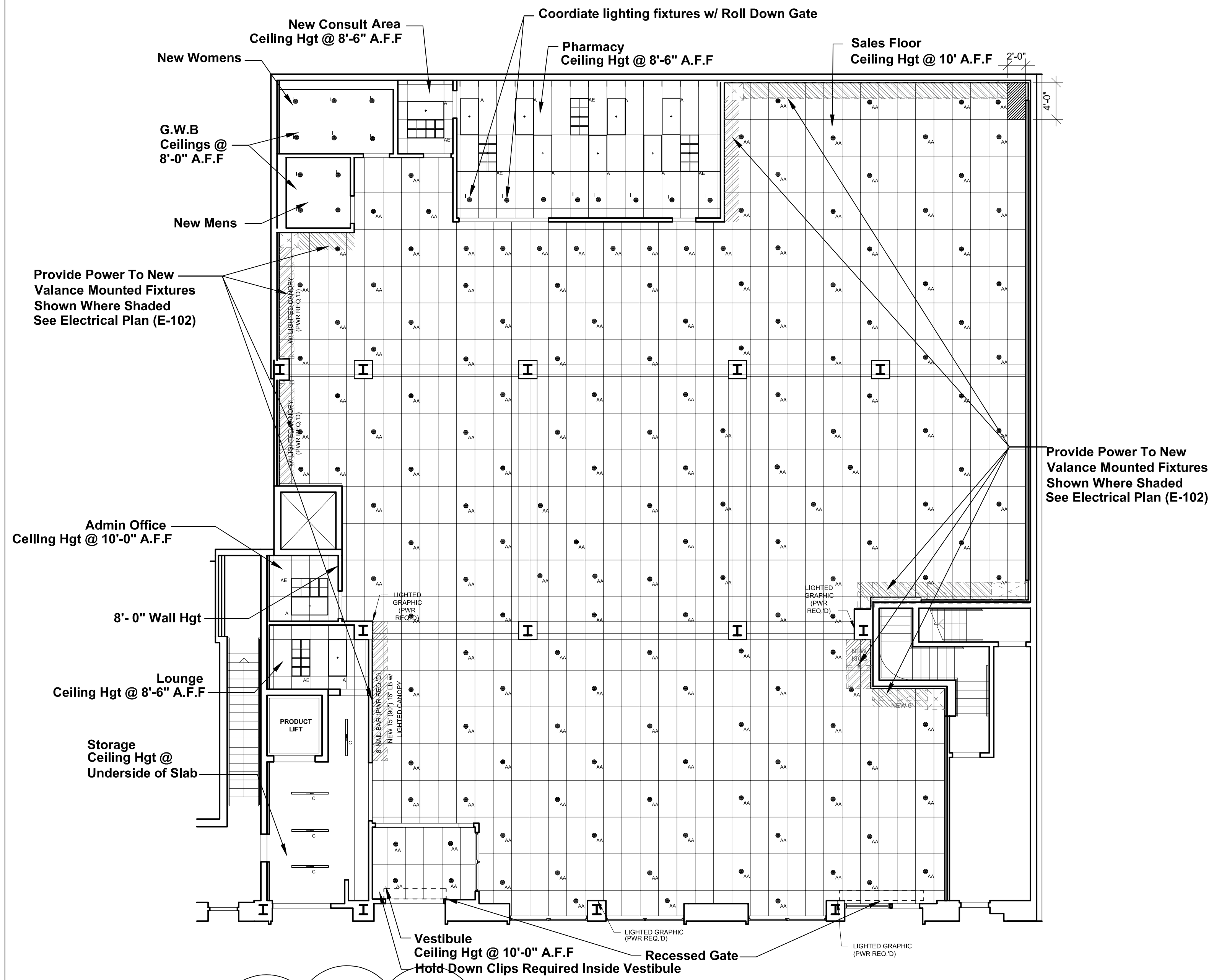
2 FIRST FLOOR REFLECTED CEILING PLAN 1/8" = 1'-0"
