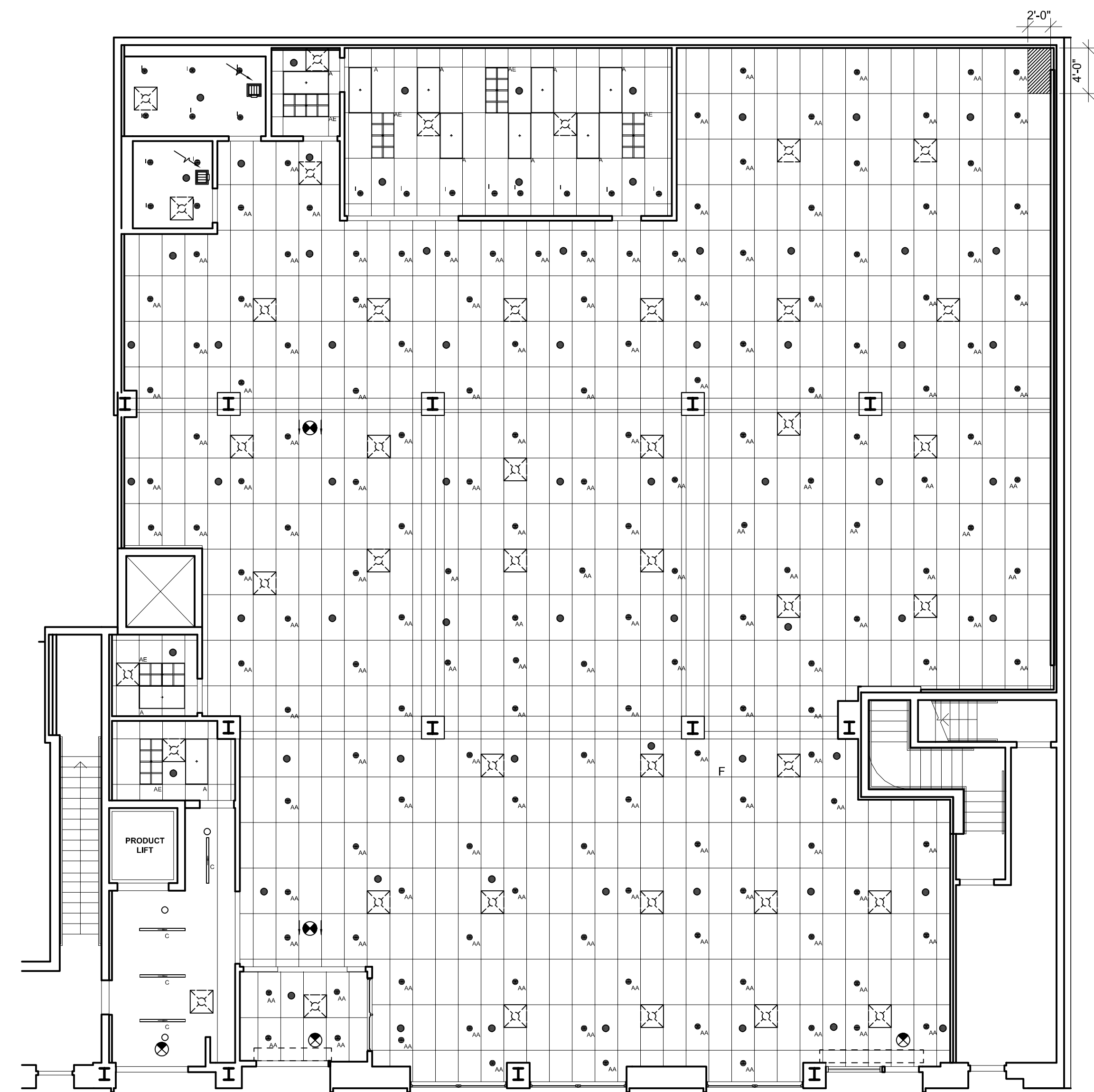
② FIRST FLOOR COORDINATED REFLECTED CEILING PLAN 1/8" = 1'-0"
