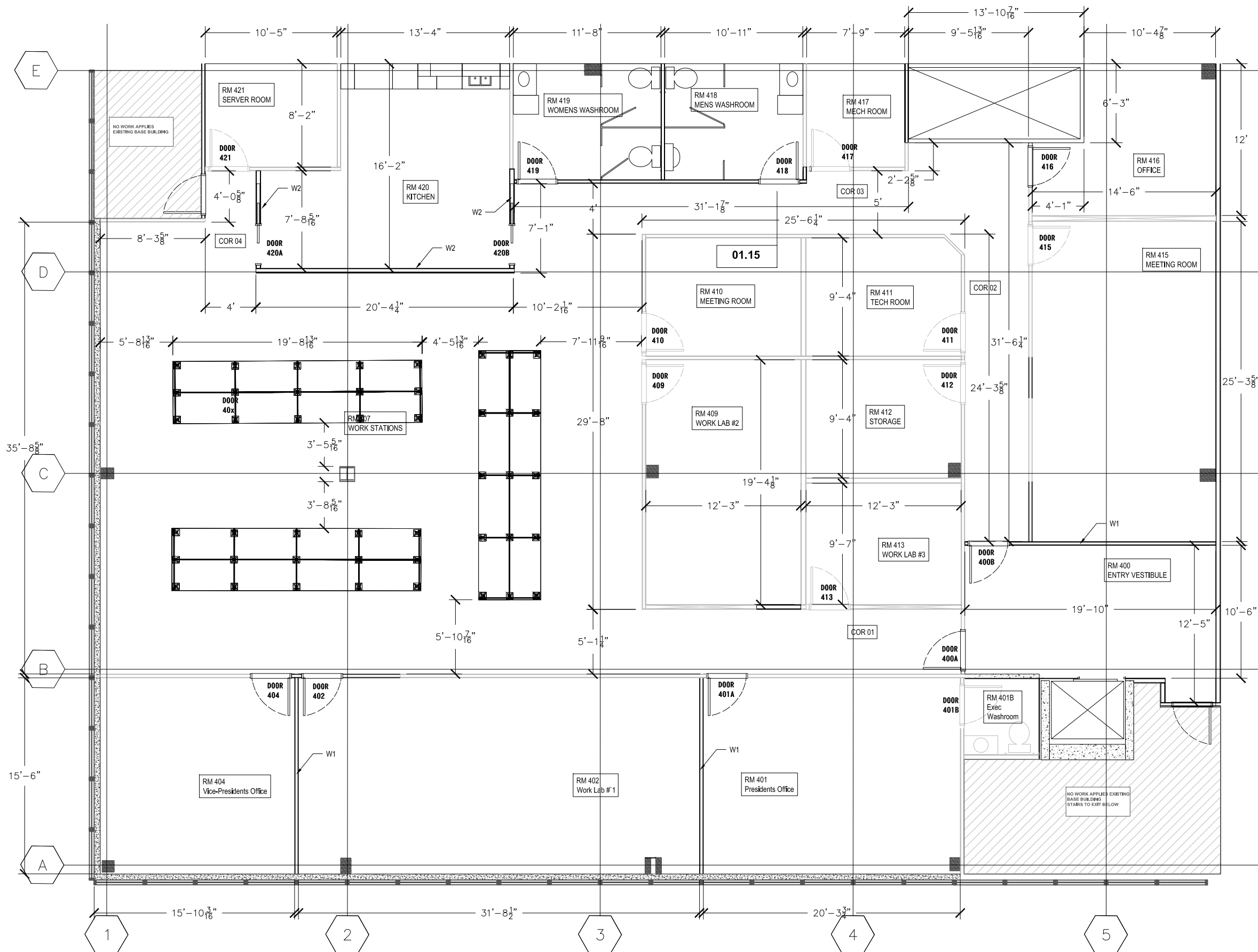
01 FLOOR PLAN - PARTITION PLAN (NEW) FURNITURE Scale (on 11x17): 1/8" = 1' - 0" - NOT AVAILABLE Scale (on 22x34): 1/4" = 1' - 0"
