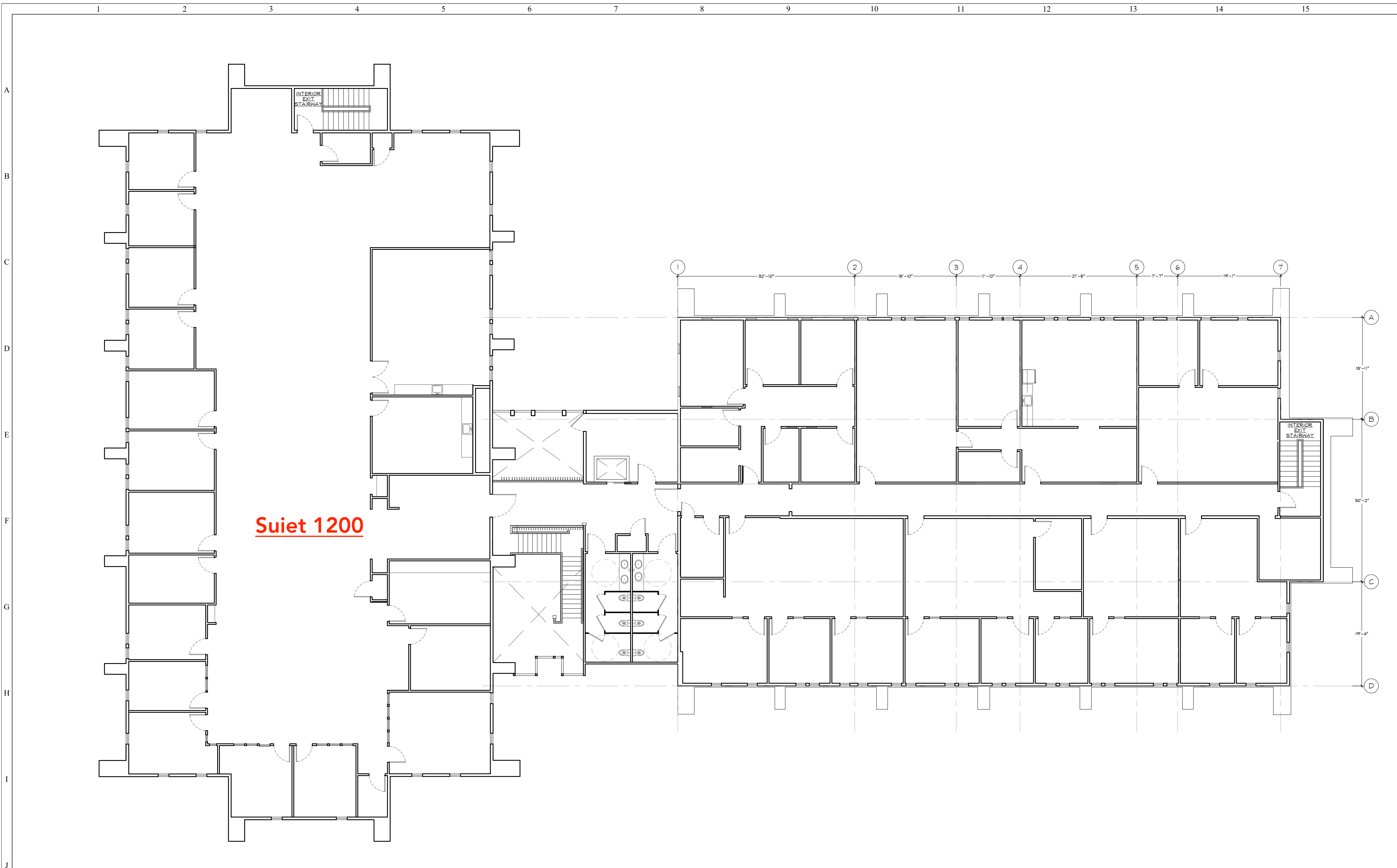
1 SECOND FLOOR PLAN 1485 CIVIC COURT SCALE: 1/8" = 1'-0" 0 2 4 8 16
