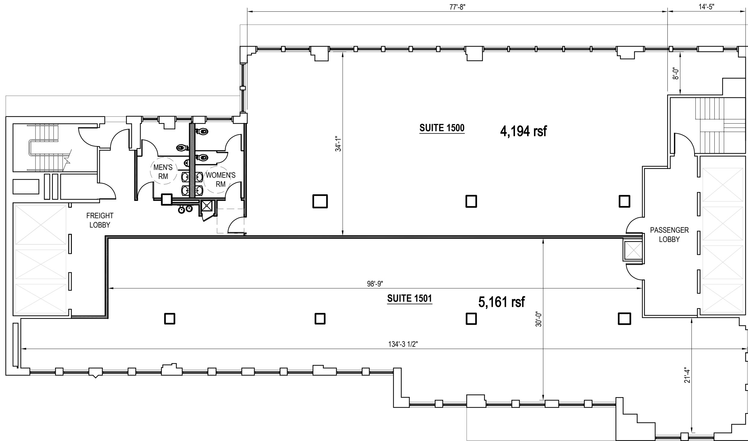
1 150 W30TH ST - 15TH FL - DEMISING PLAN - SCHEME B SCALE: 3/32" = 1'-0"
