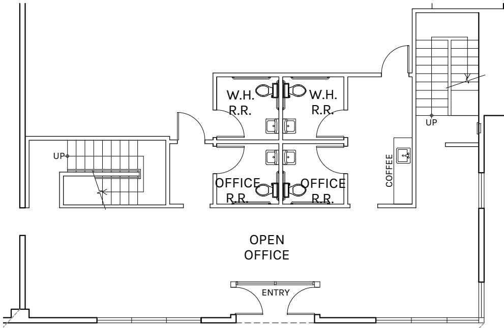
02 GROUND LEVEL OFFICE
