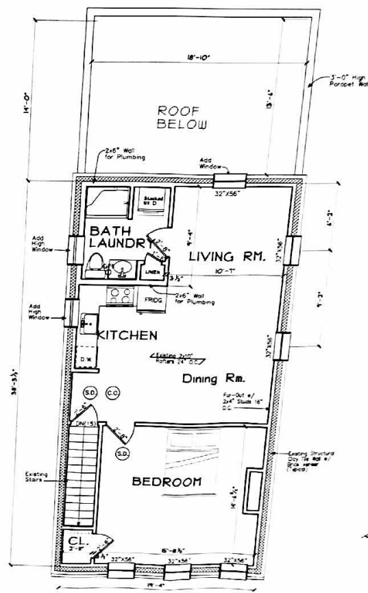
2 Level Two Plan A2.02
