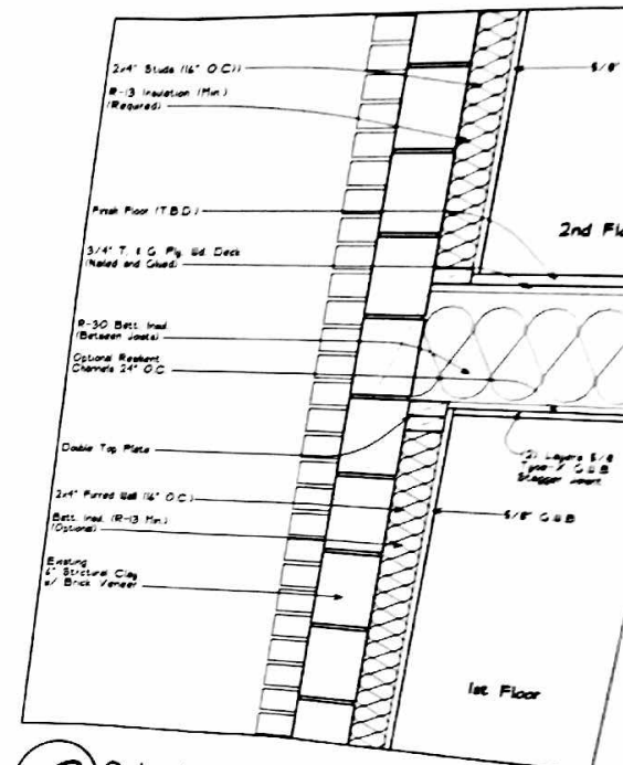
3 Ceiling/Wall Detail FEET 2
