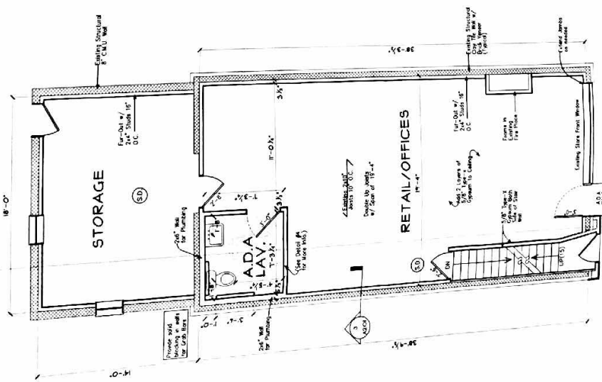
1 Level One Plan A2.01
