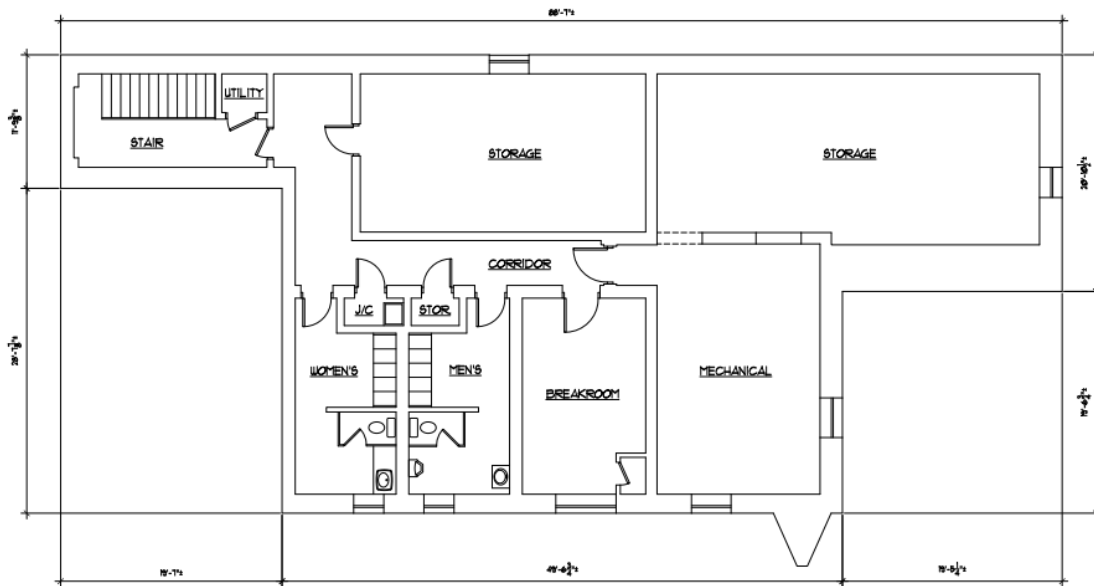
EXISTING LOWER LEVEL PLAN RENTABLE AREA = 2,695 SF
