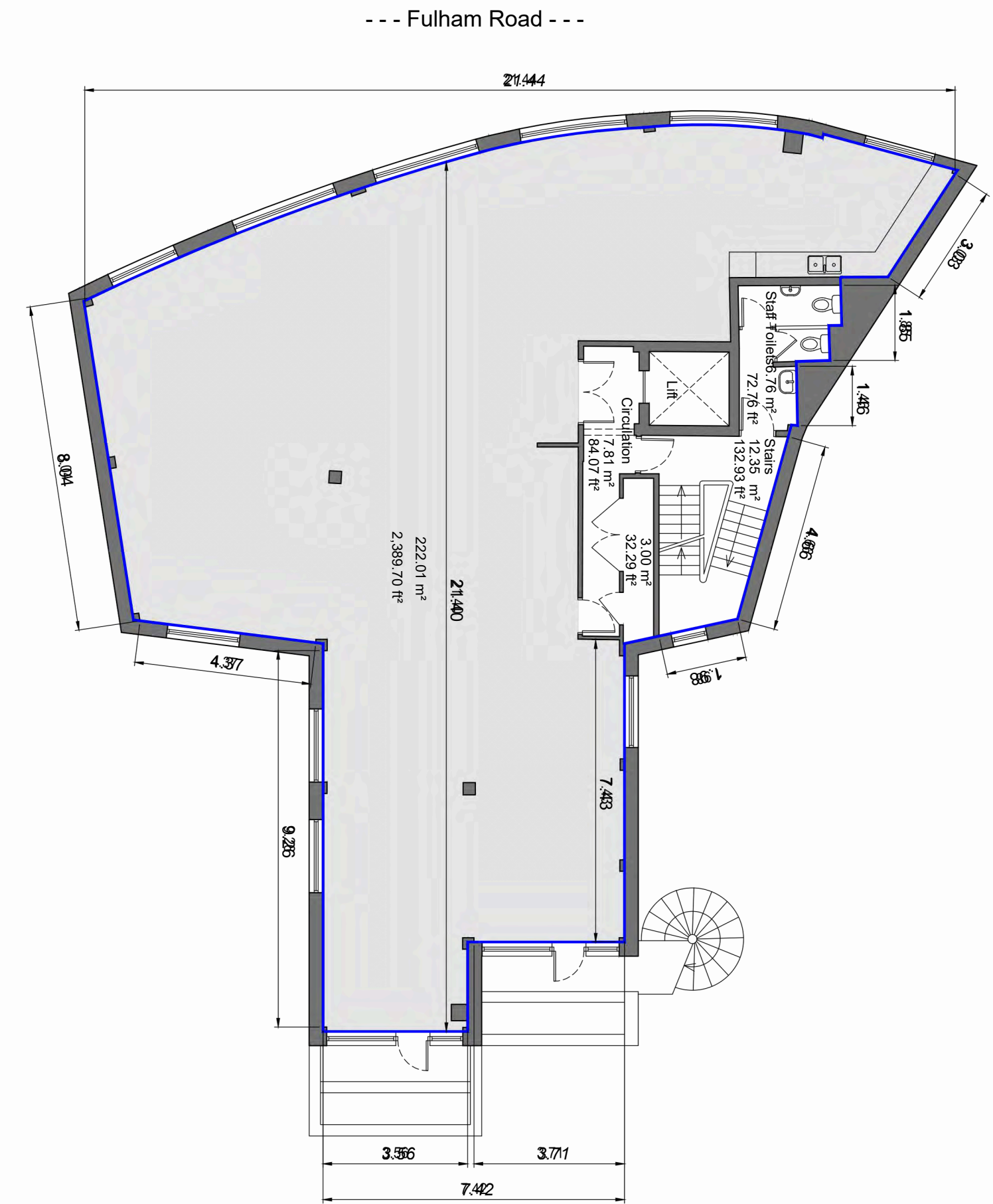
SECOND FLOOR Office 2,390 sq ft / 222.01 sq m
