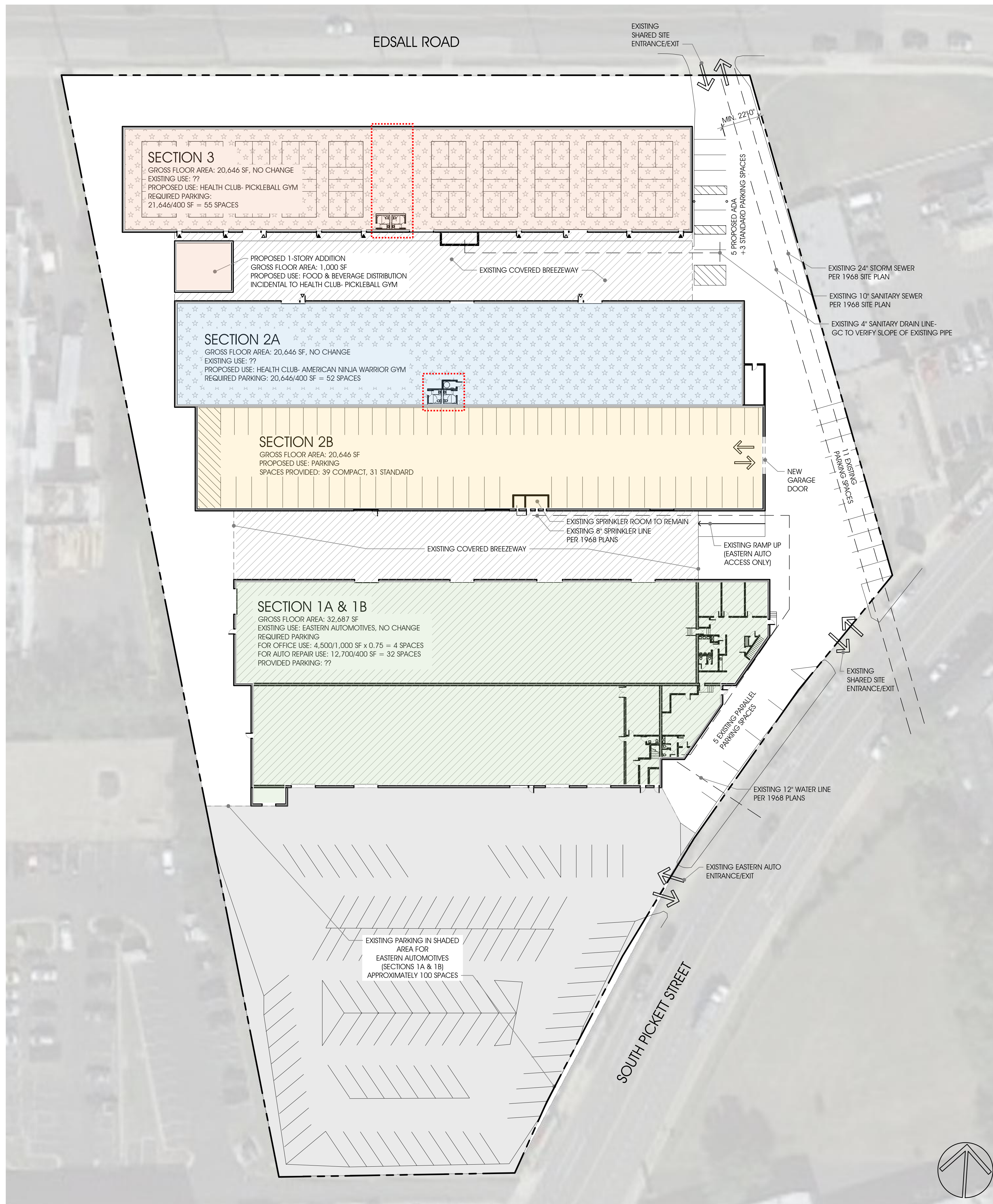
OVERALL BUILDING PLAN 1/32" = 1'-0"
