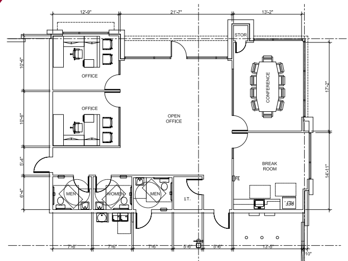
1,609 SF OFFICE PLAN
