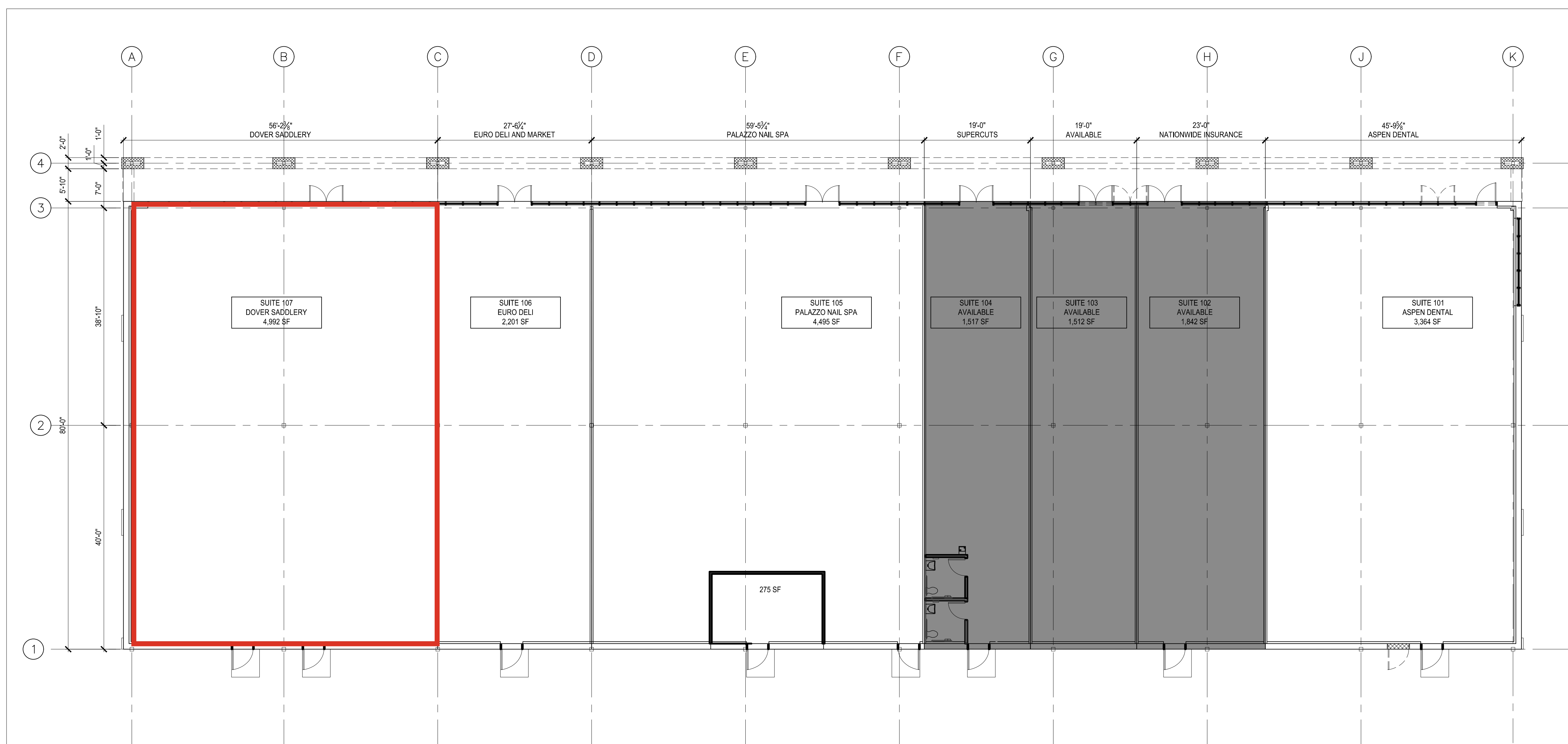
FLOOR PLAN
