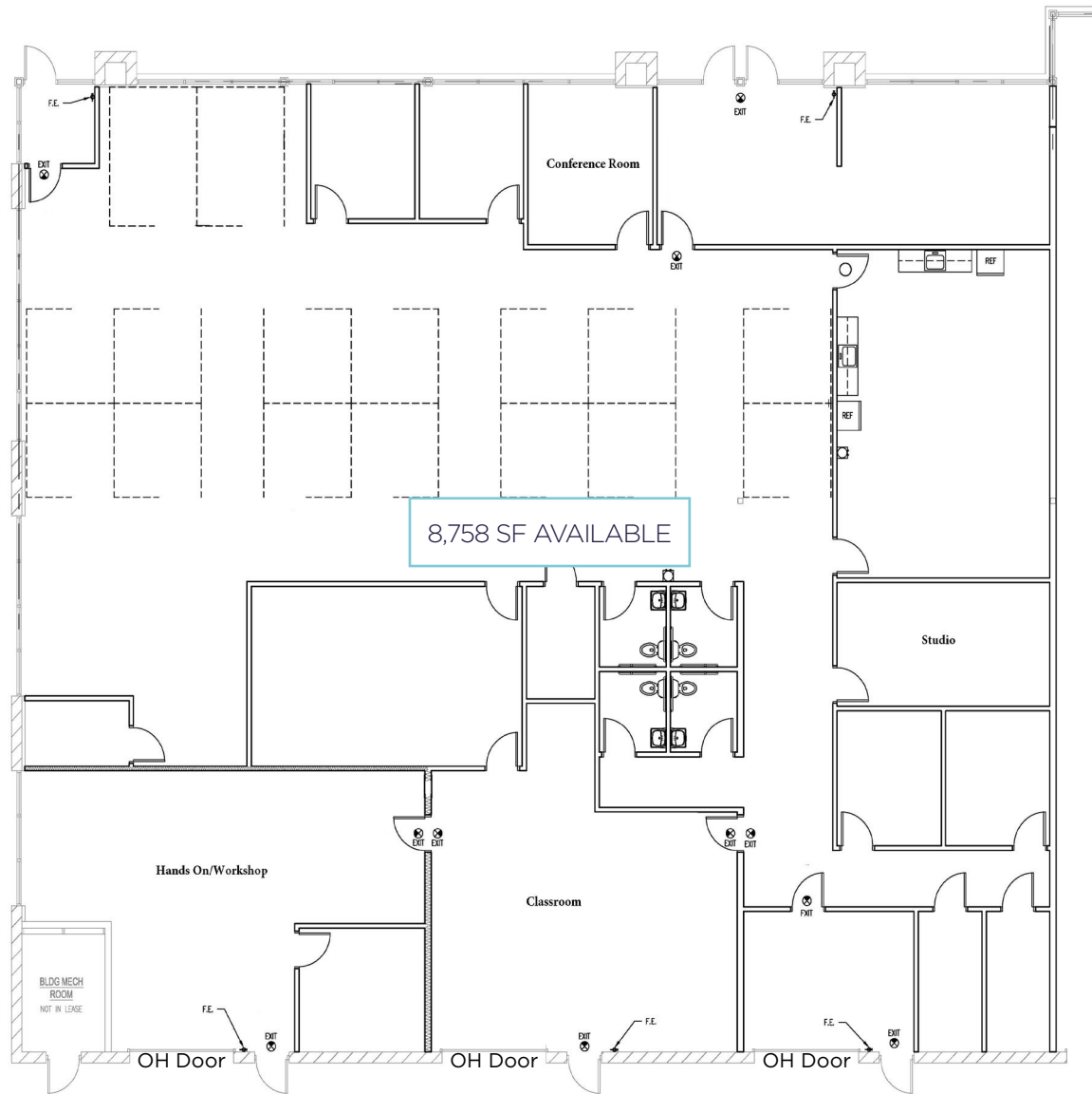
1 FLOOR PLAN 3/16" = 1'-0"
