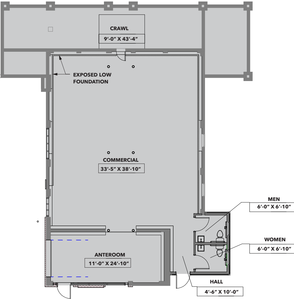
BASEMENT- 1,868 GSF
