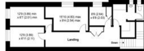
SECOND FLOOR
