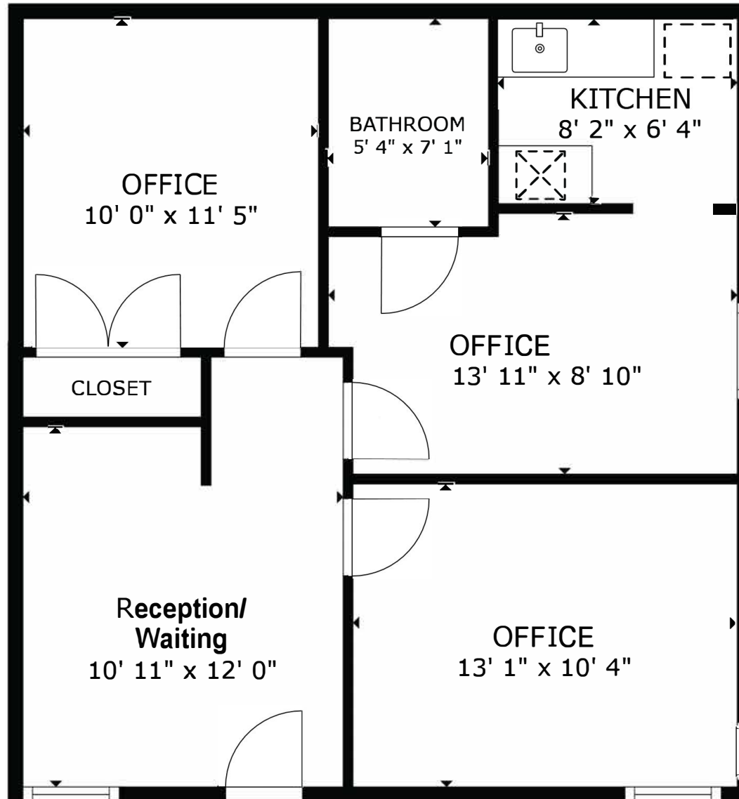
FLOOR PLAN
