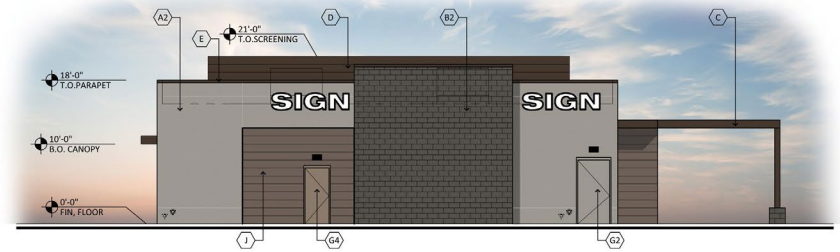
SHOPS A - EAST ELEVATION
