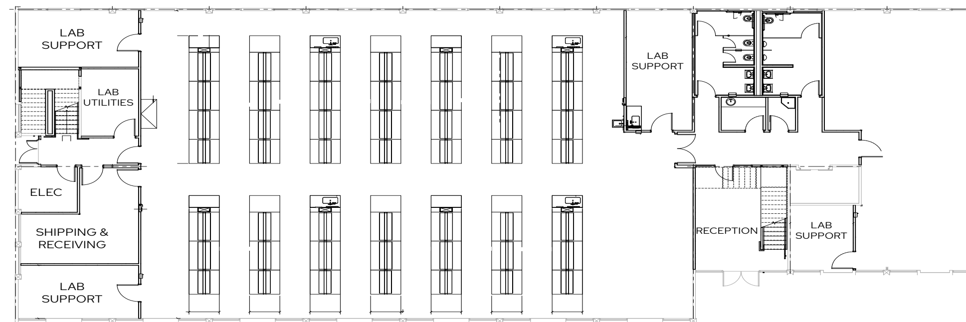
First Floor
