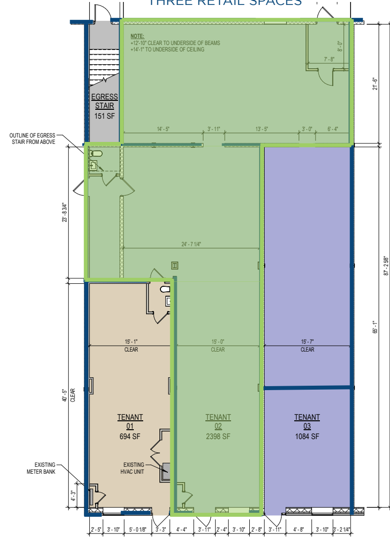
OPTION 2 THREE RETAIL SPACES
