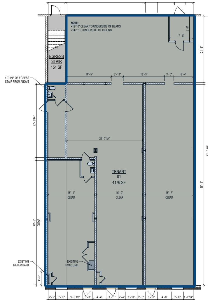
OPTION 4 Entire 4,176 SF Ground Floor
