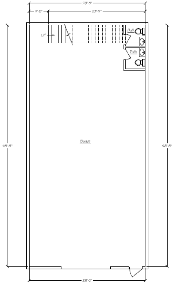
1st Level Proposed Scale: 1/8" = 1'0"
