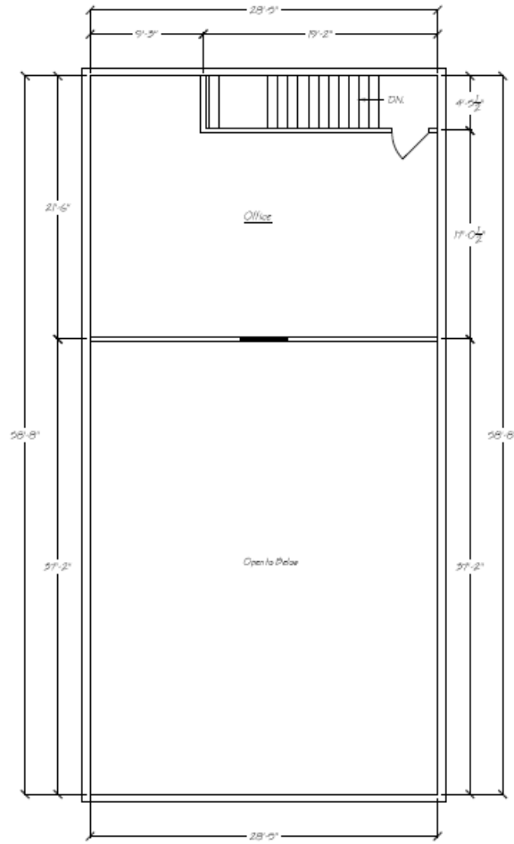
2nd Level Proposed Scale: 1/8" = 1'0"
