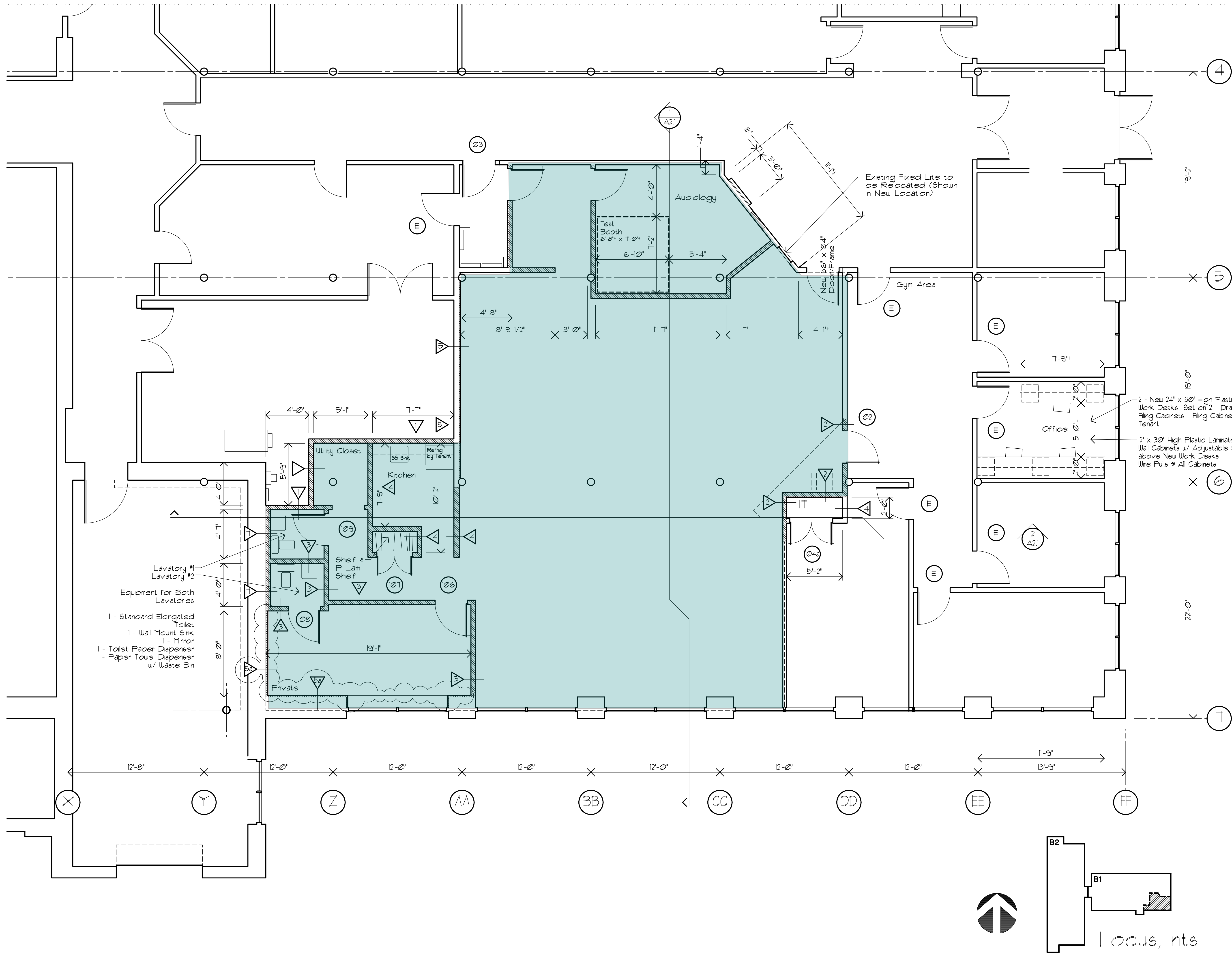
1 Partial First Floor Plan - BI-FI, 1/4" = 1'-0"
