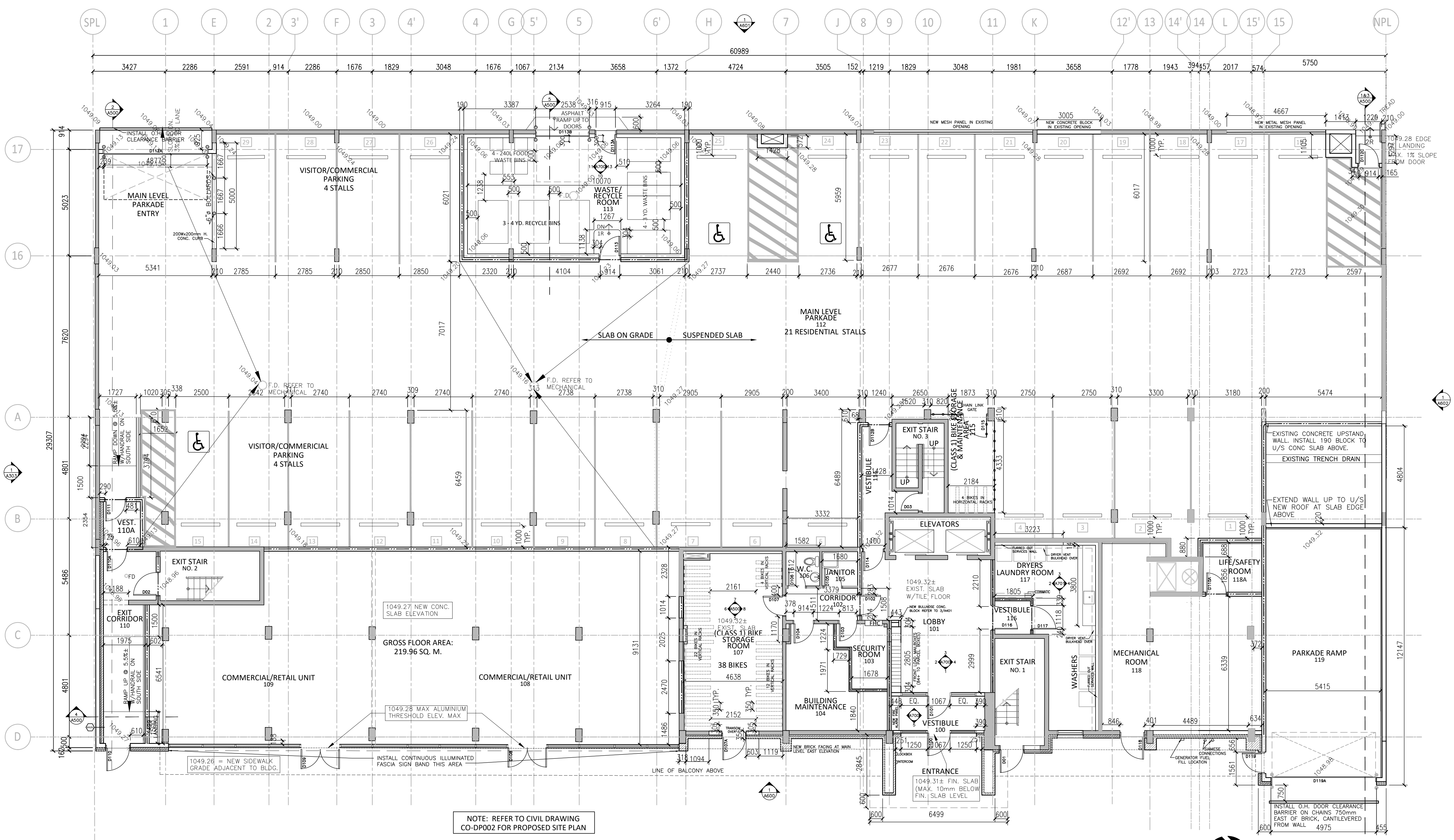
1 MAIN FLOOR PLAN GRADES A-100 SCALE = 1 : 100
