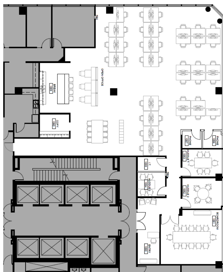
East Views
