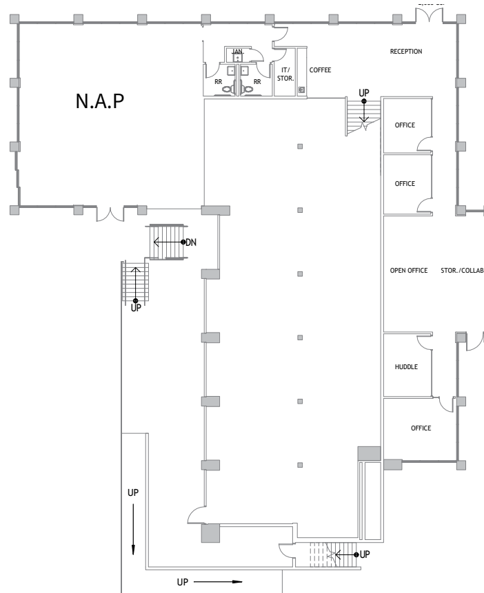
LEVEL 2
