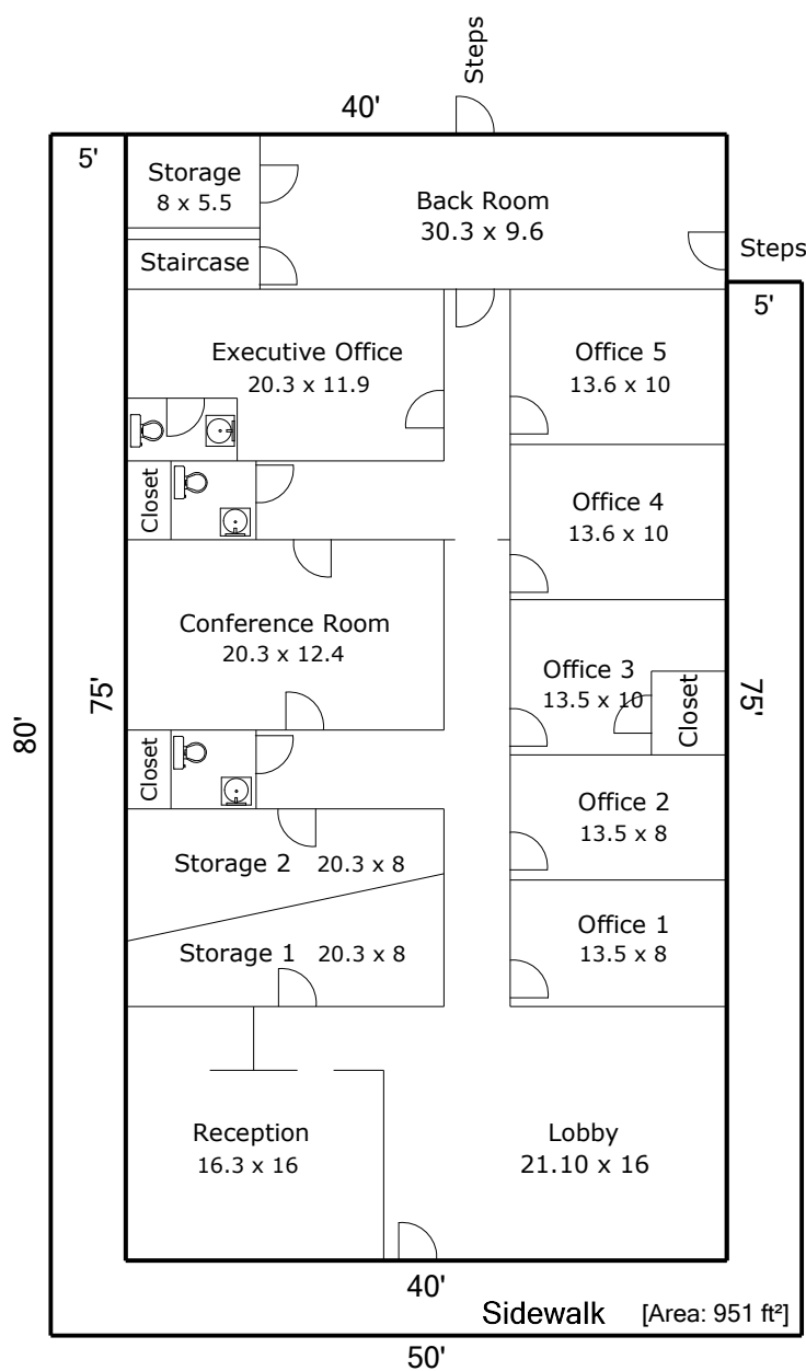
First Floor [Area: 3000 ft²]
