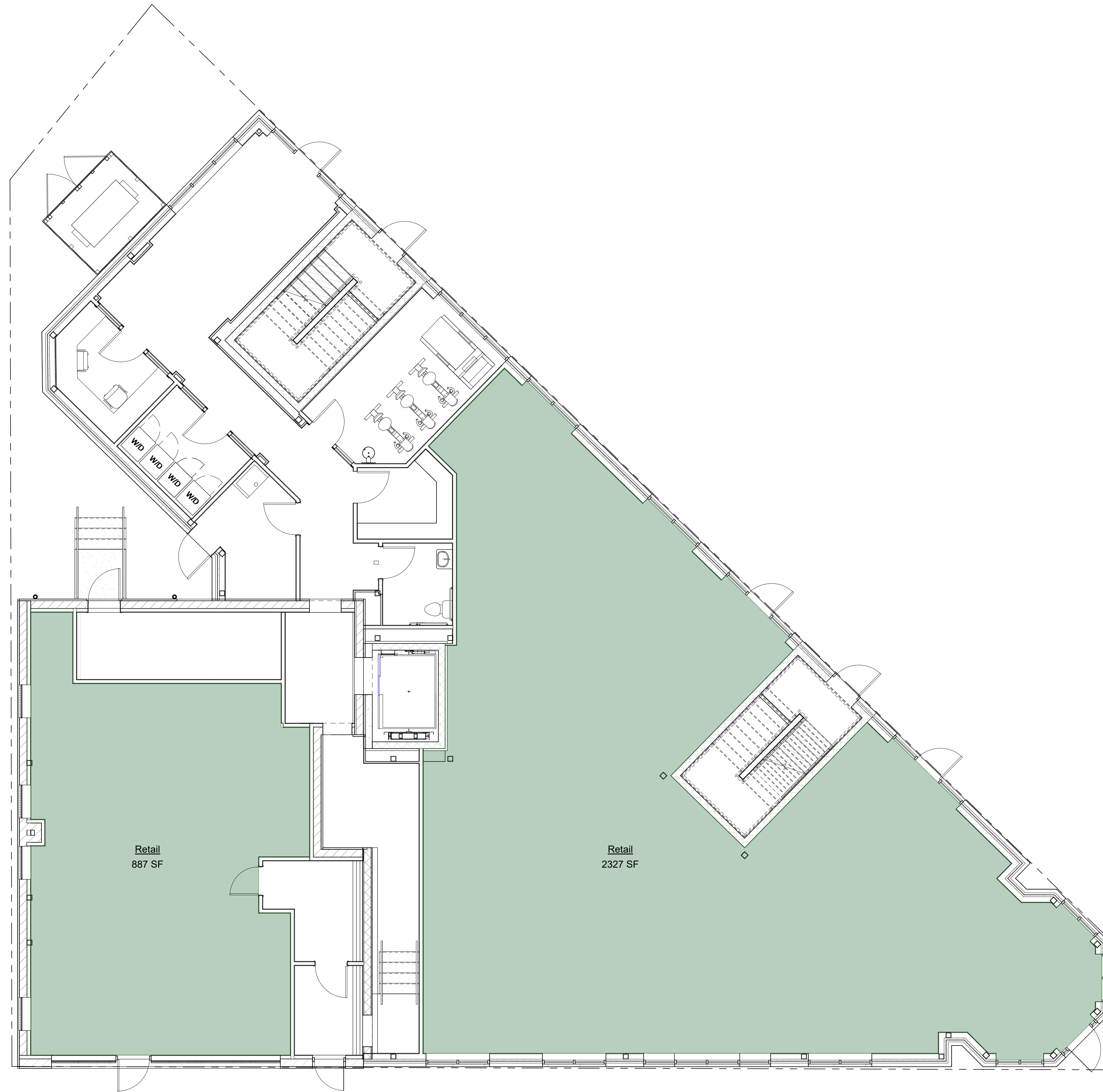
Arrowhead Residential & Retail Facility 1355 Main Street, Hartford, Connecticut First Floor Net Area Plan
