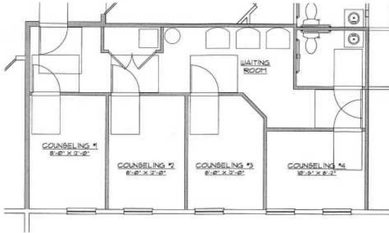
TEST FIT FLOOR PLAN #2 1/4" = 1'-0"
