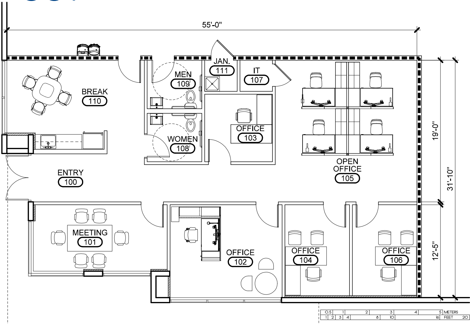
ENLARGED OFFICE PLAN
