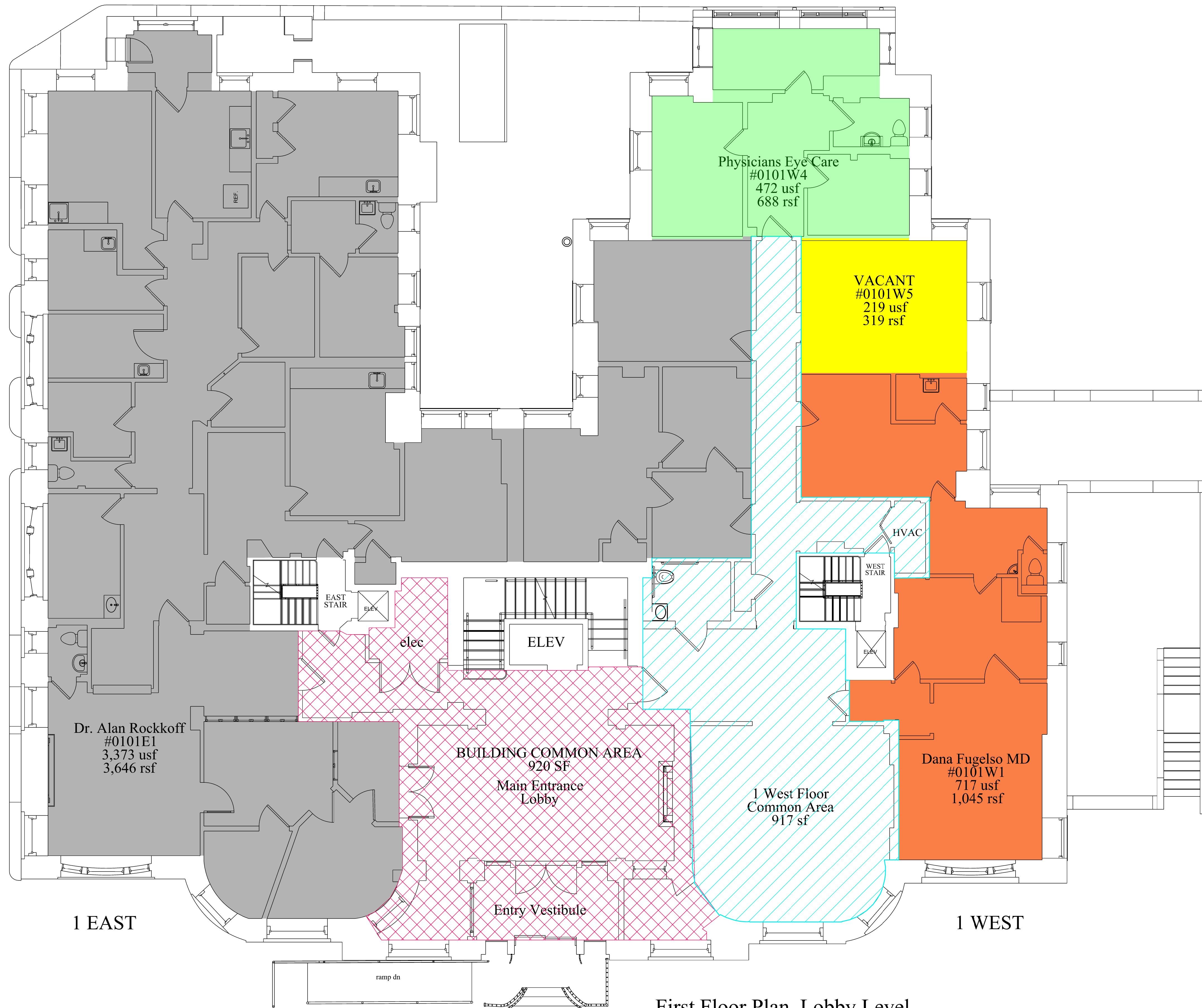
1 First Floor Plan, Lobby Level 3/16" = 1'-0"
