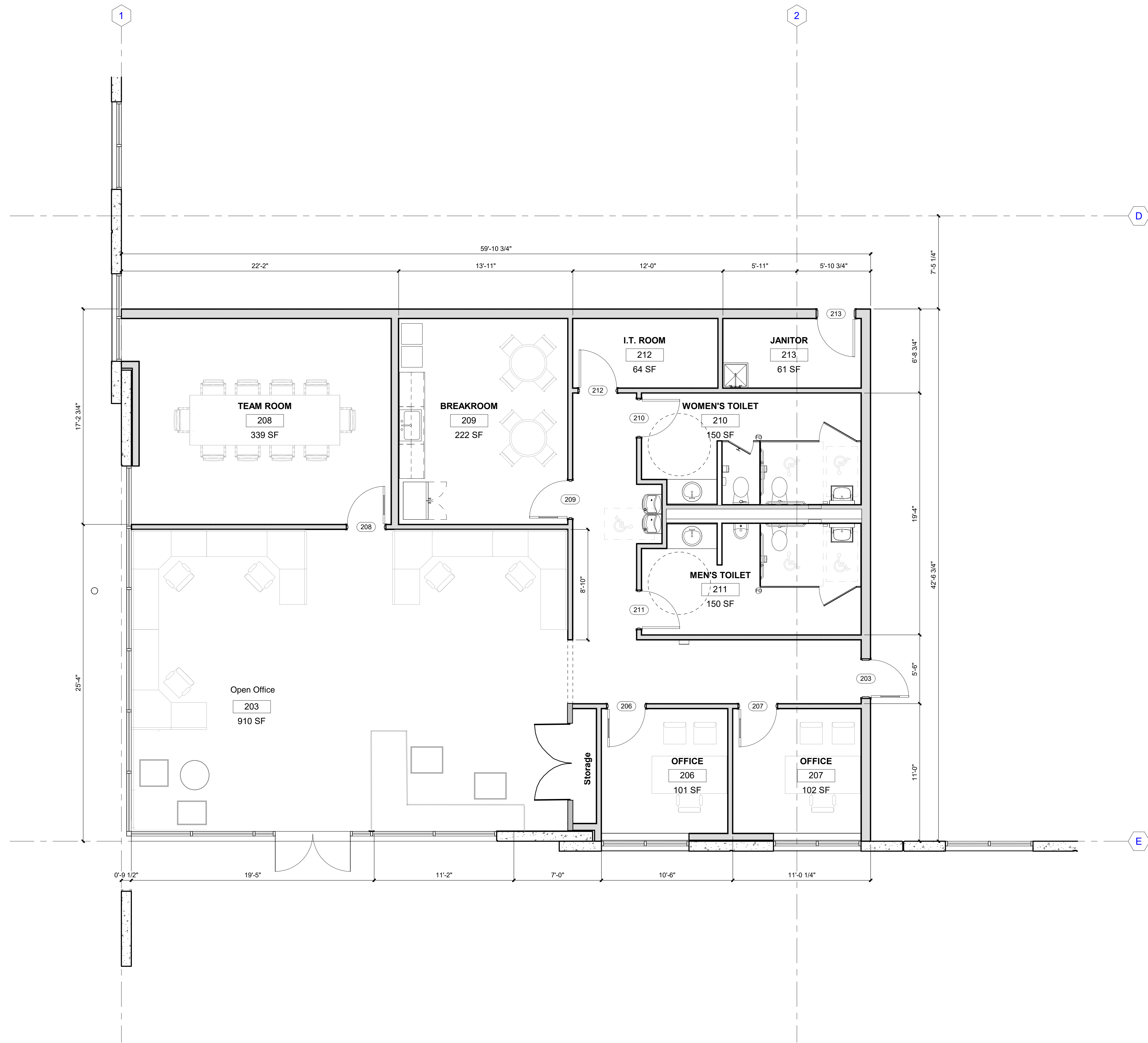
1 OFFICE PLAN 2,543 SF A110 SCALE: 1/4" = 1'-0"
