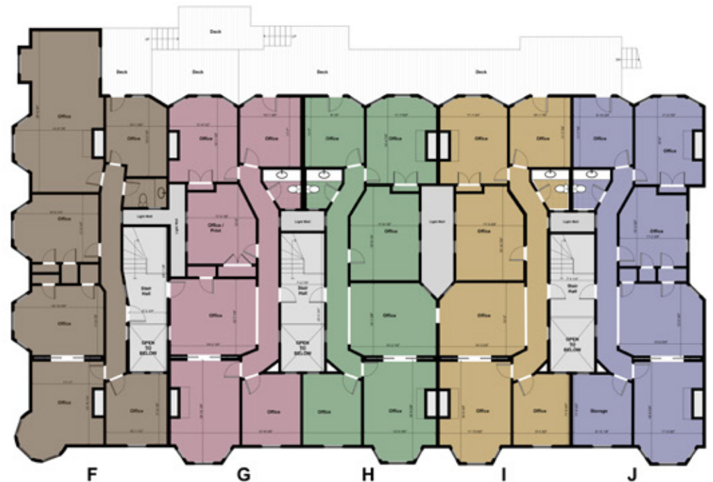
3RD FLOOR
