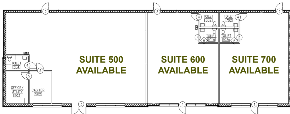
2 Floor Plan — Building 2 1/8" = 1'-0"
