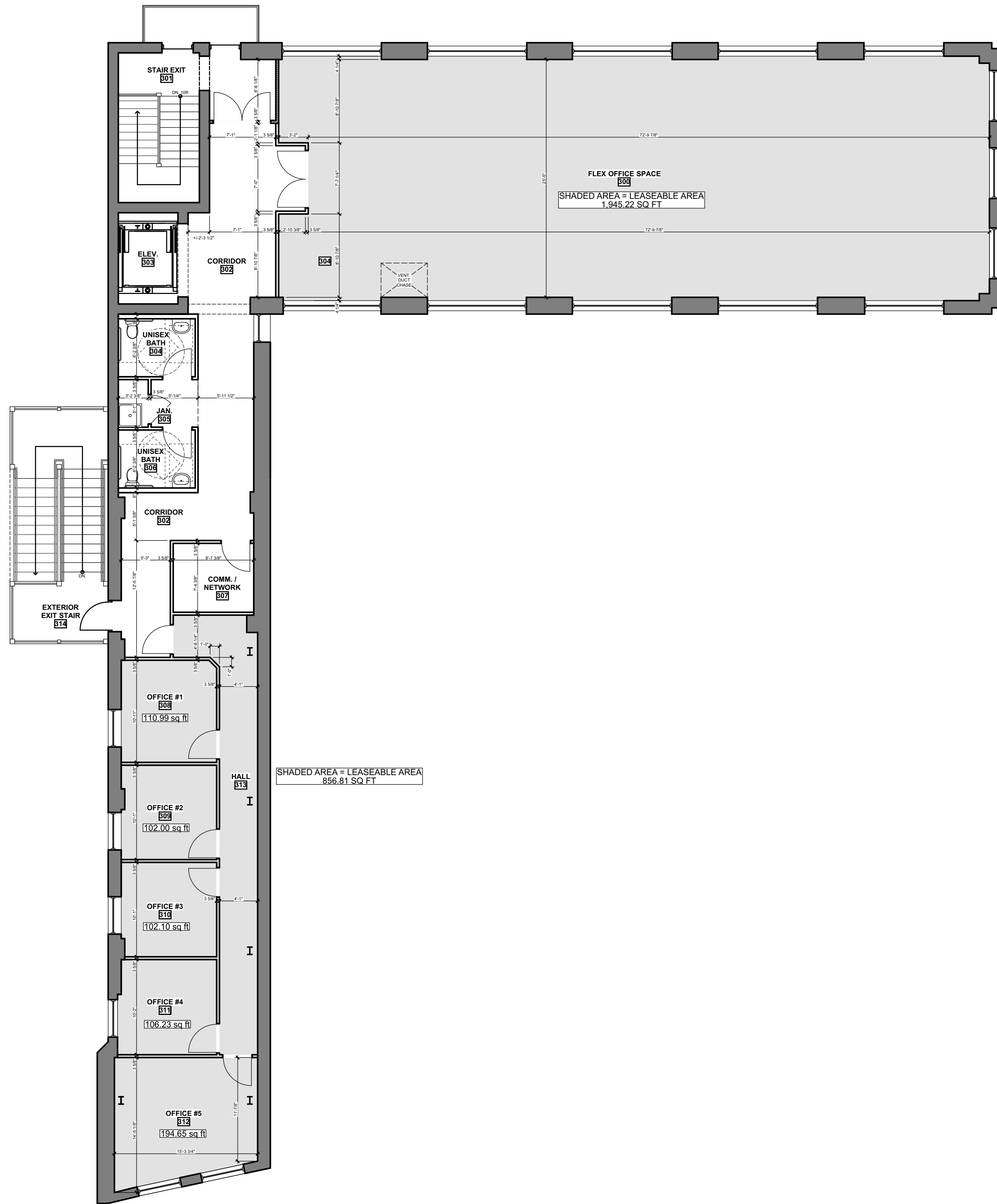
2 PROPOSED THIRD FLOOR MARKETING PLAN MK-101 SCALE: 1/8" = 1'-0"
