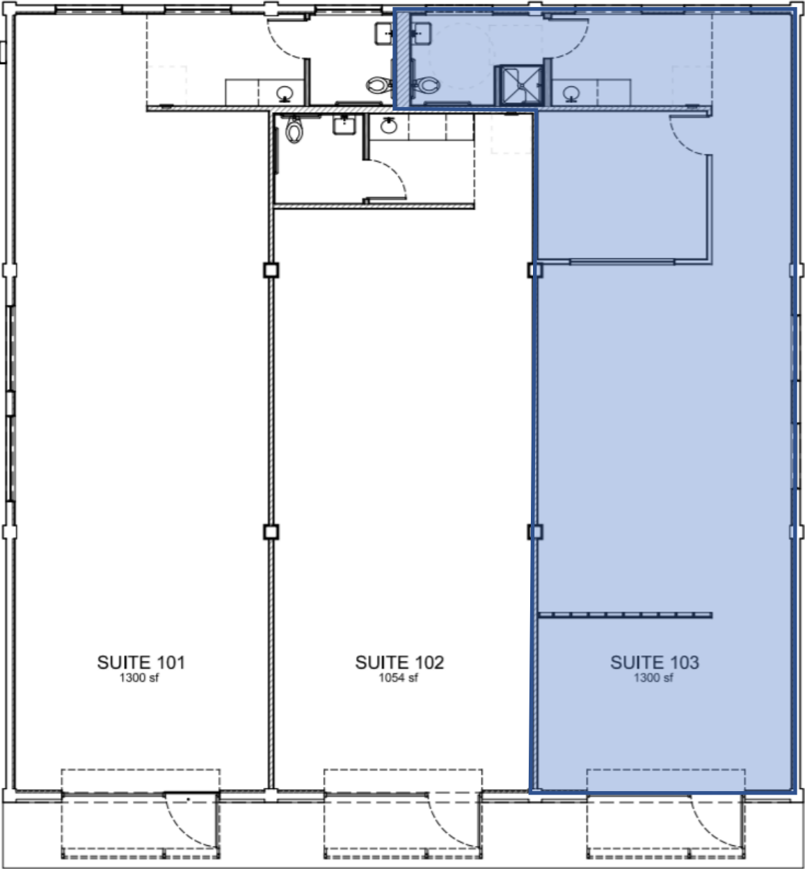
1 BUILDING #5: Floor Plan Scale: 1/8" = 1'-0"
