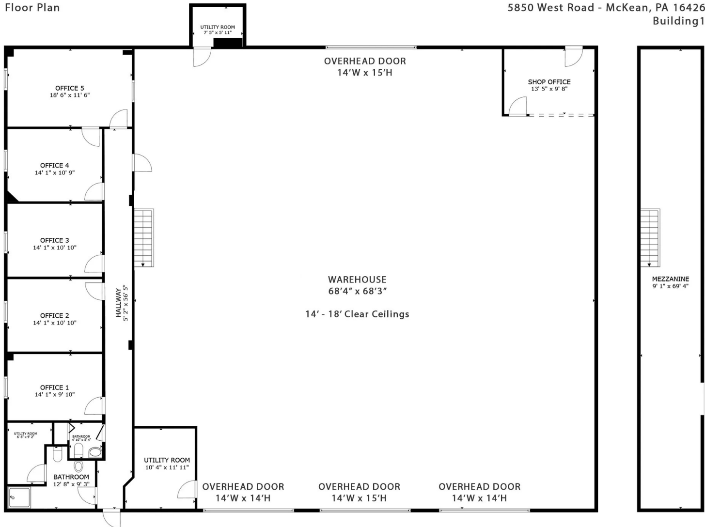
Floor Plan
