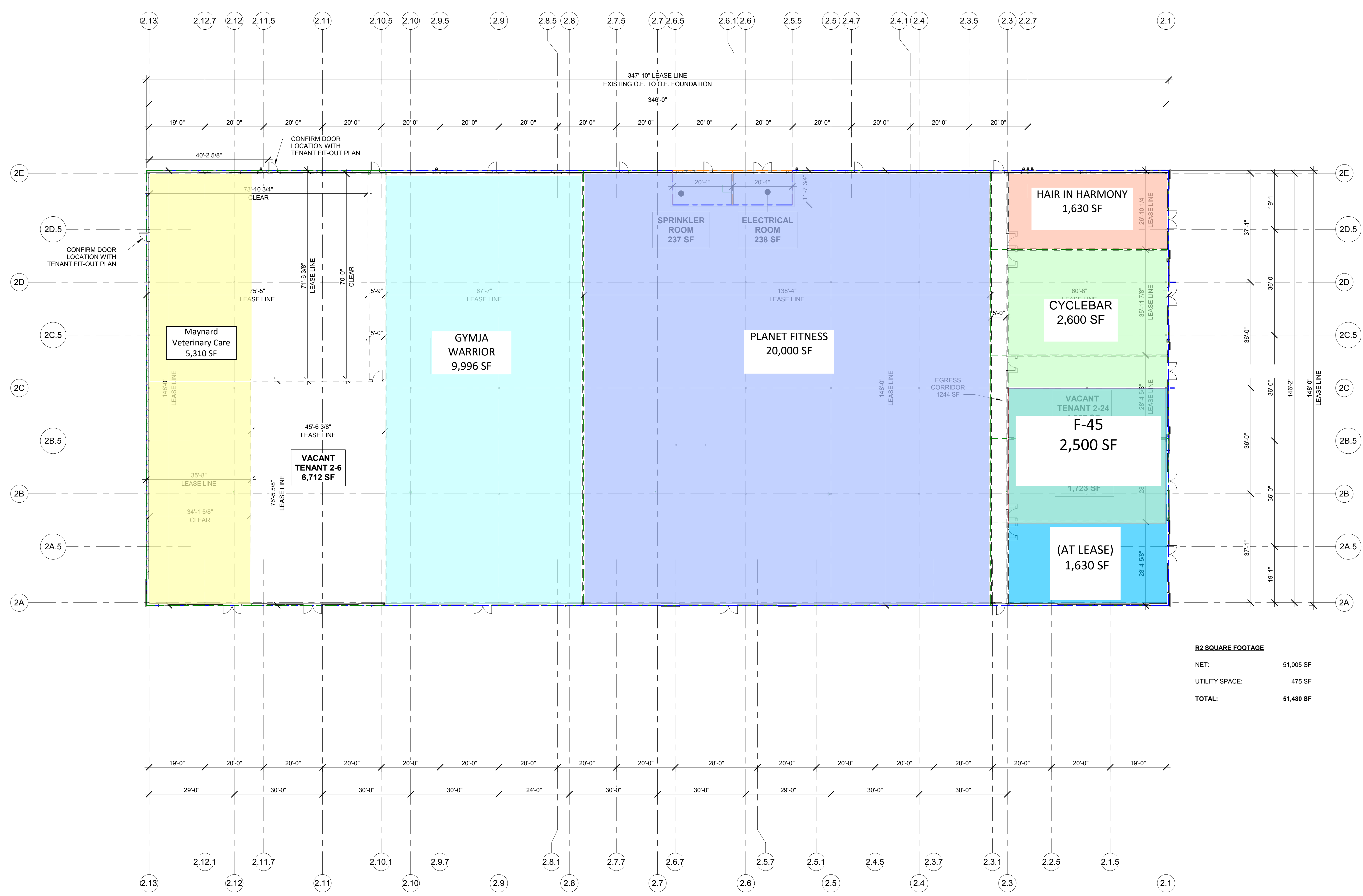
1 BUILDING R2 A2 1/16" = 1'-0"
