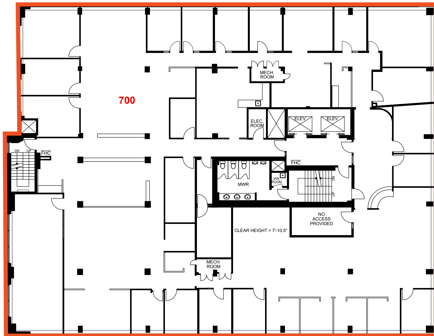
Existing Floor Plan - Suite 700 (Full Floor)
