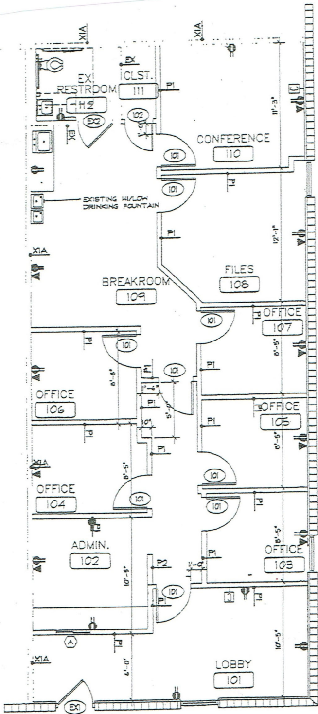
1 FLOOR PLAN SCALE: 1/4" = 1'-0"
