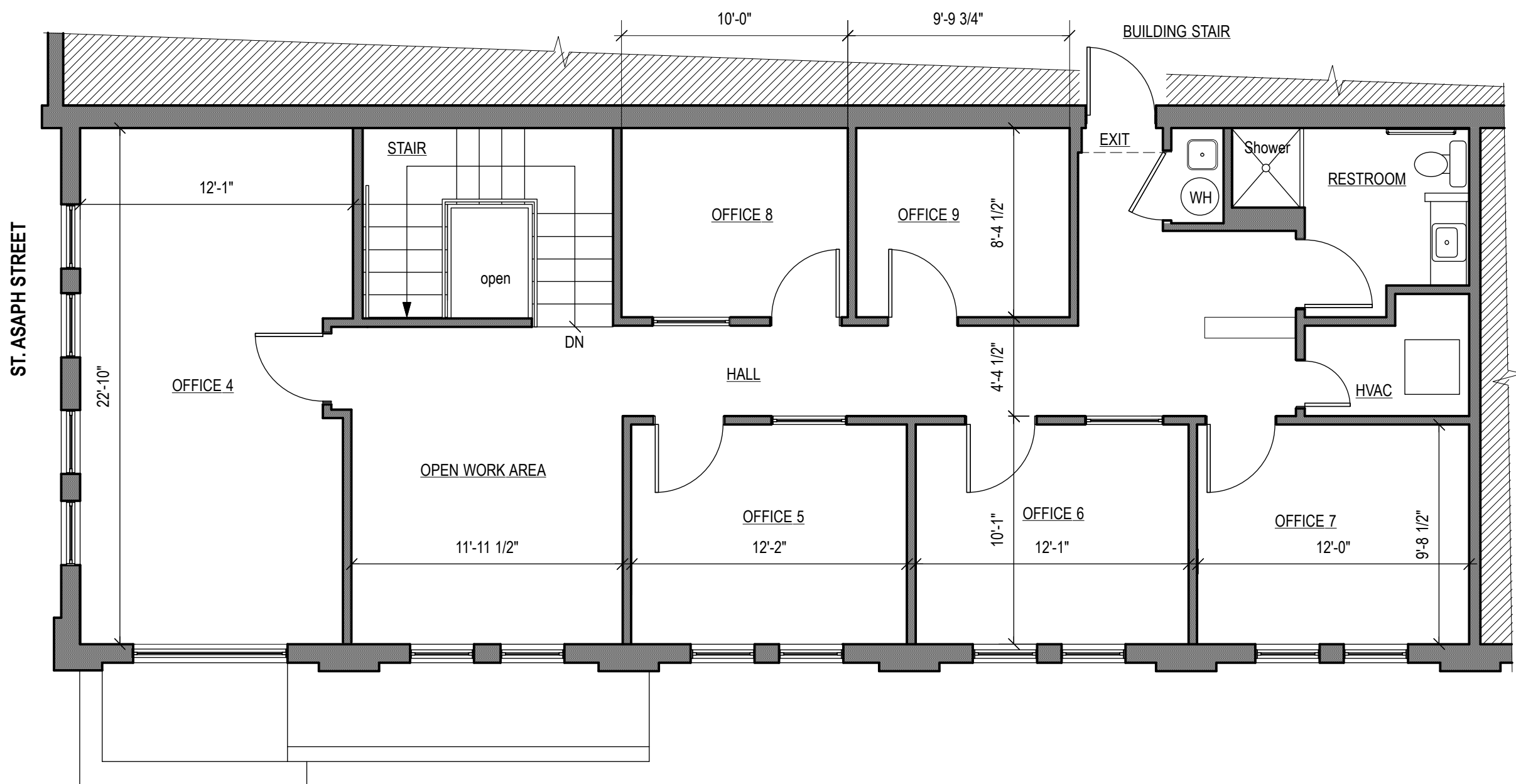
2 SECOND FLOOR PLAN Scale: 3/16" = 1'-0"
