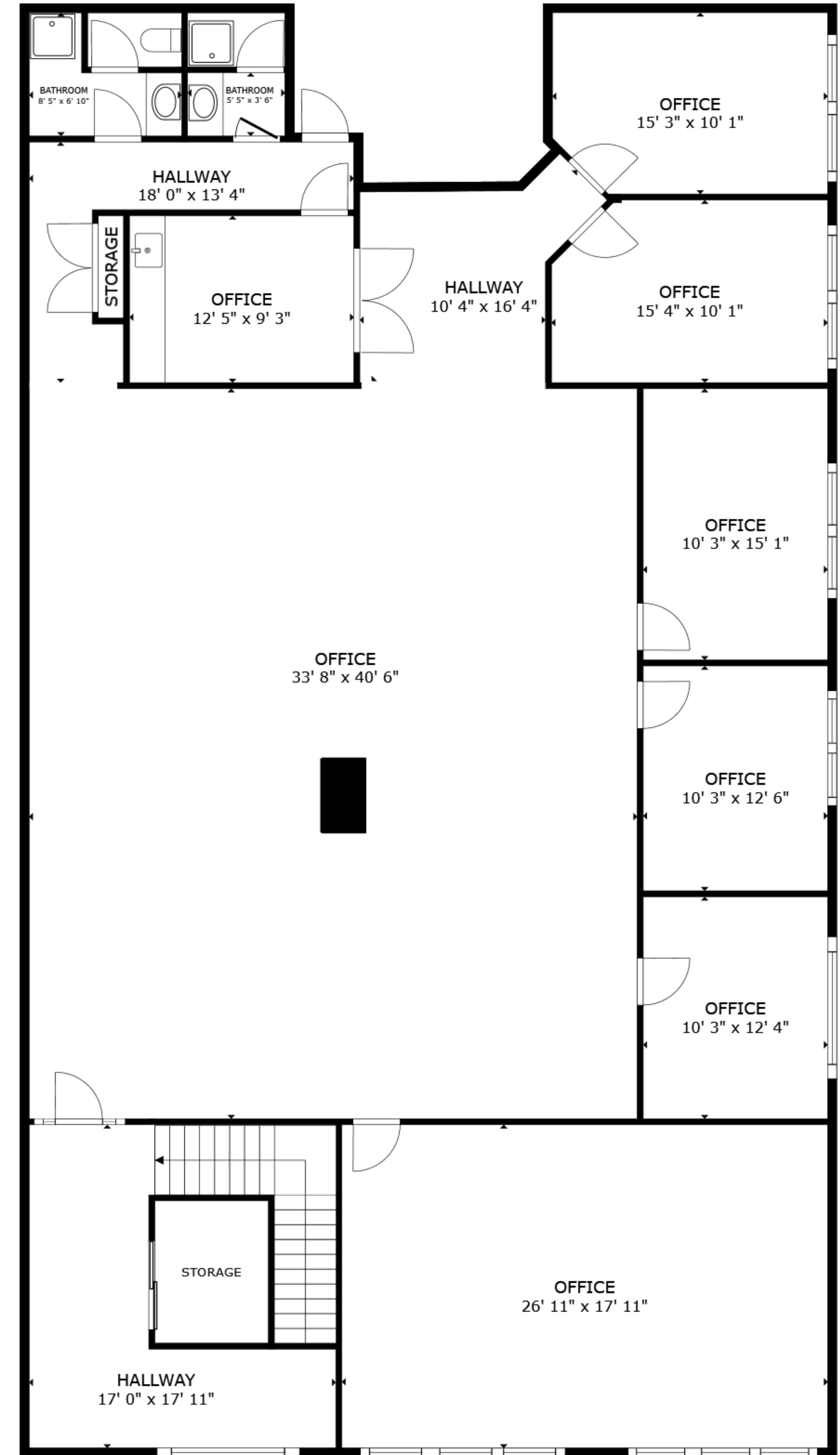
FLOOR 3
