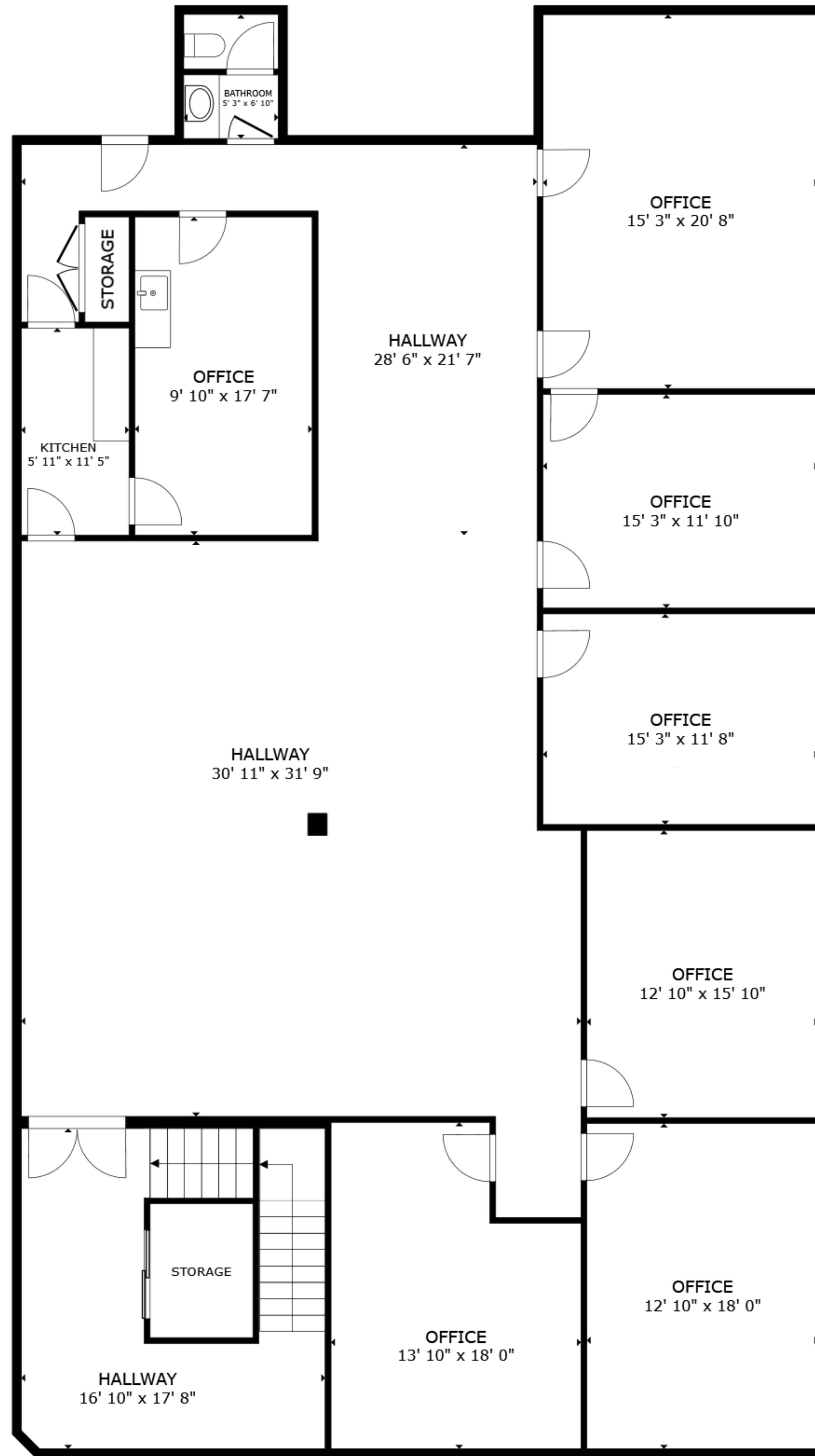
FLOOR 2
