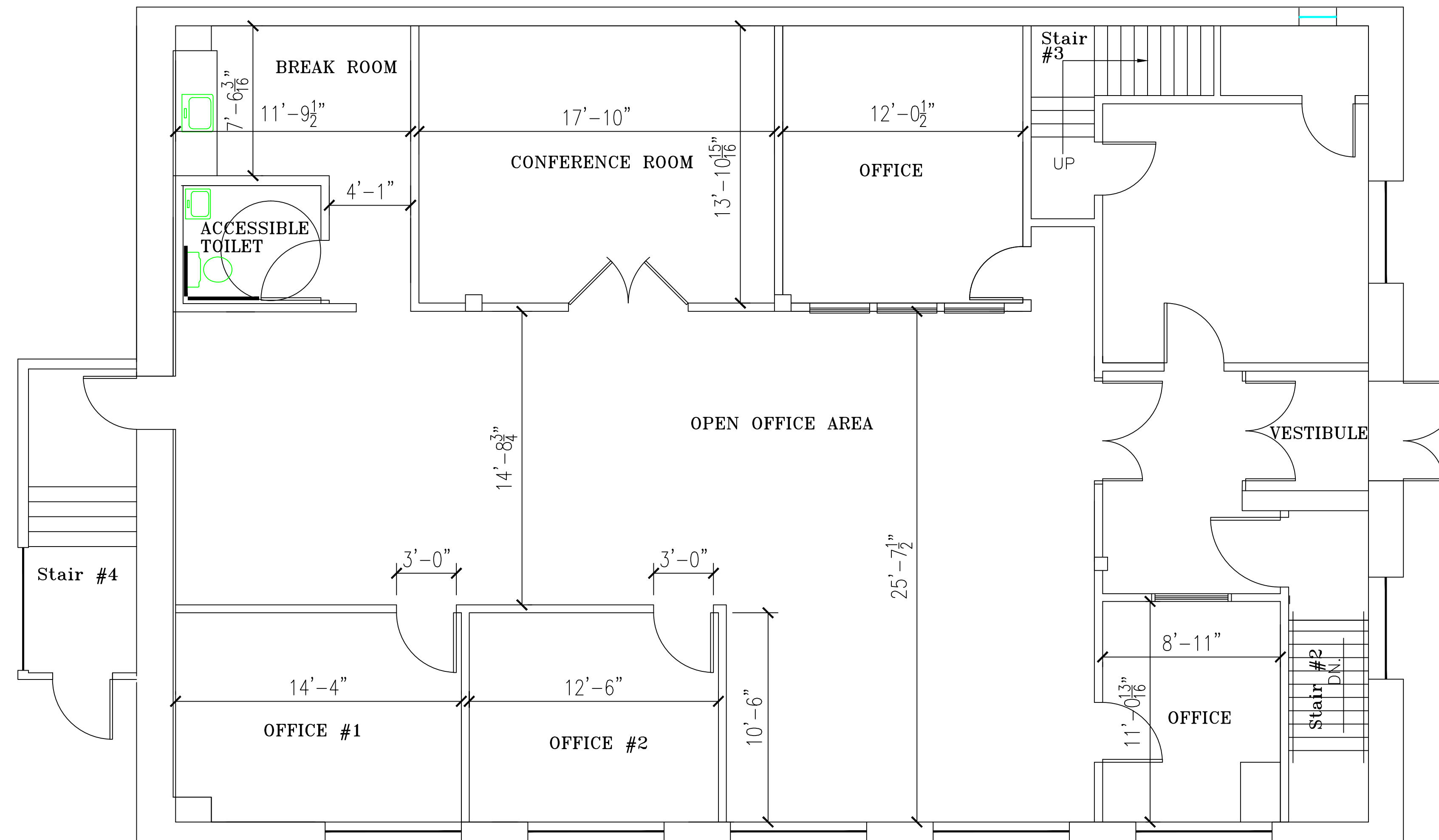
PROPOSED FIRST FLOOR PLAN SCALE: 1/4"=1'-0"
