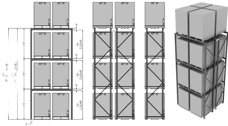
64" Tall Pallets, 30' Clear 3,004 Total Pallet Positions
