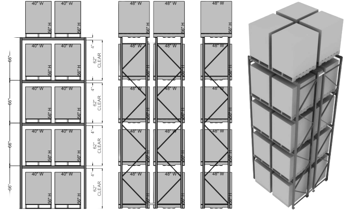
56" Tall Pallets, 30' Clear 3,788 Total Pallet Positions
