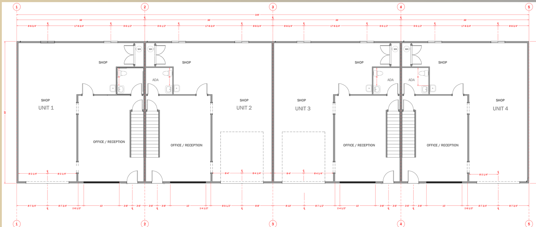
MAIN FLOOR PLAN
