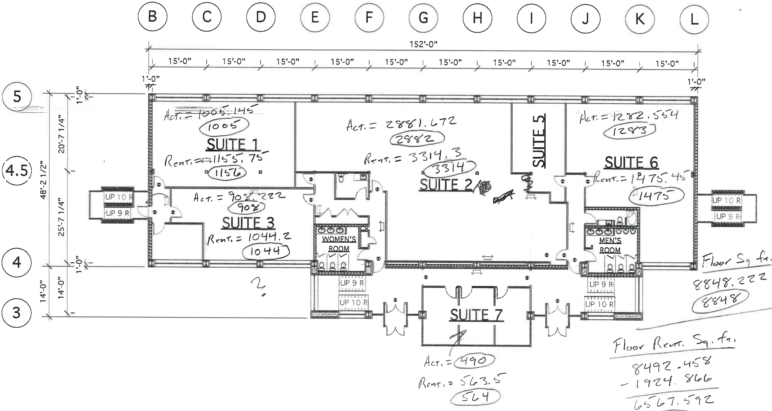
1 LOWER LEVEL FLOOR PLAN A-1 Scale: 1/16" = 1'-0" NOTE: ALL DIMENSIONS ARE TO BE VERIFIED IN THE FIELD.
